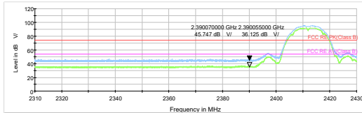
802.11b-Channel 1 Peak+ Average
