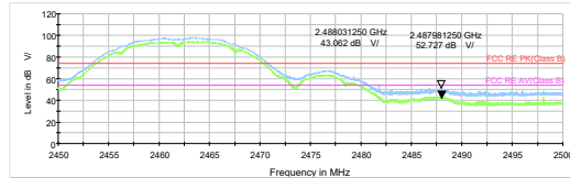
802.11b-Channel 11 Peak+ Average
