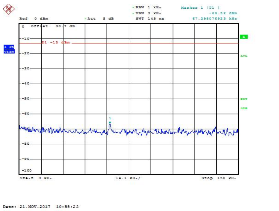
Figure 8 - 159.0000 MHz - 9 kHz to 150 kHz
