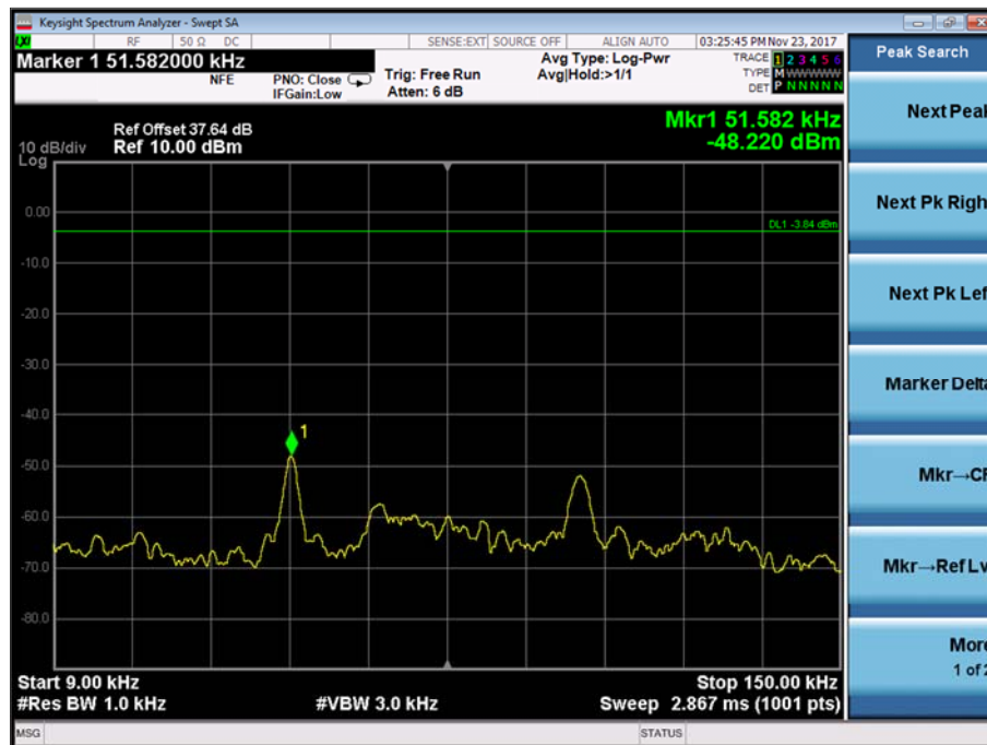
Figure 23 - 9 kHz to 150 kHz
