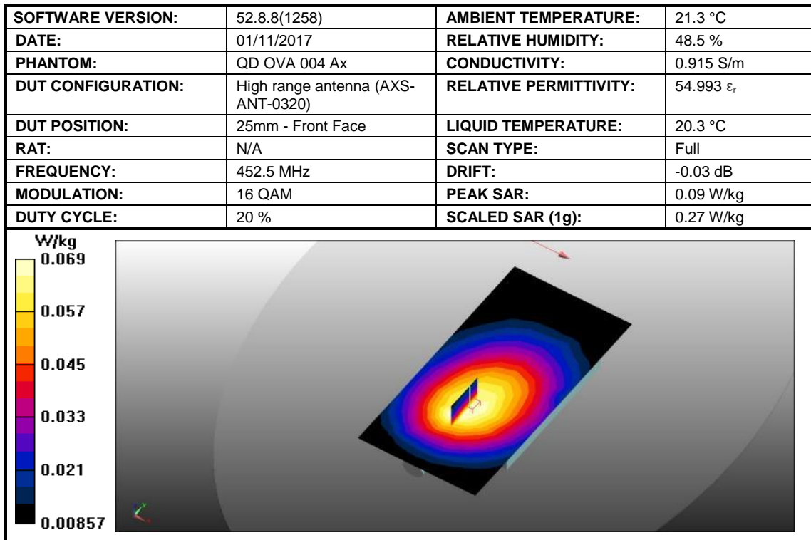
Figure 4: SAR Head Testing Results for PNG MP50 Transceiver at 452.5 MHz.
