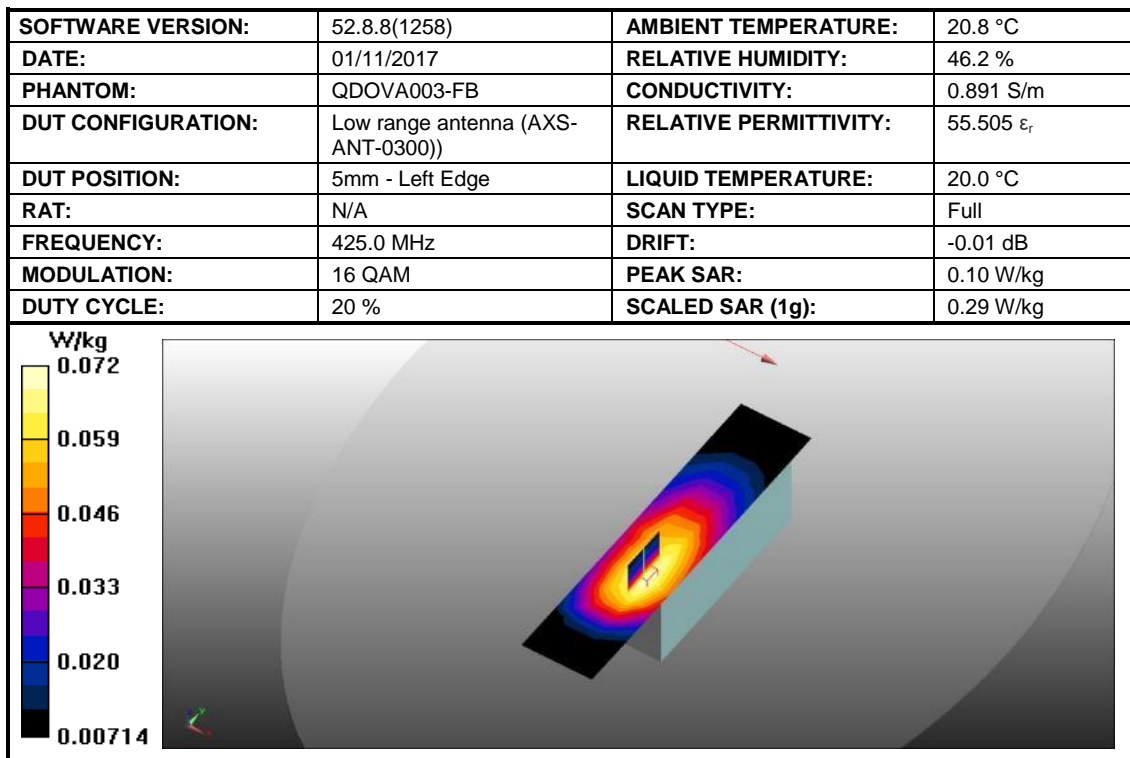
Figure 7: SAR Body Testing Results for PNG MP50 Transceiver at 425.0 MHz.
