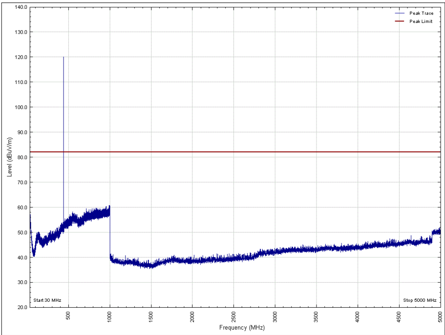
Figure 8 - 438.0500 MHz - 30 MHz to 5 GHz Vertical, EUT Orientation X
