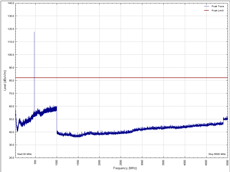
Figure 14 - 469.9875 MHz - 30 MHz to 5 GHz Vertical, EUT Orientation X
