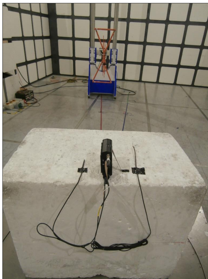
Figure 25 - Test Setup - 30 MHz to 1 GHz, Z Orientation
