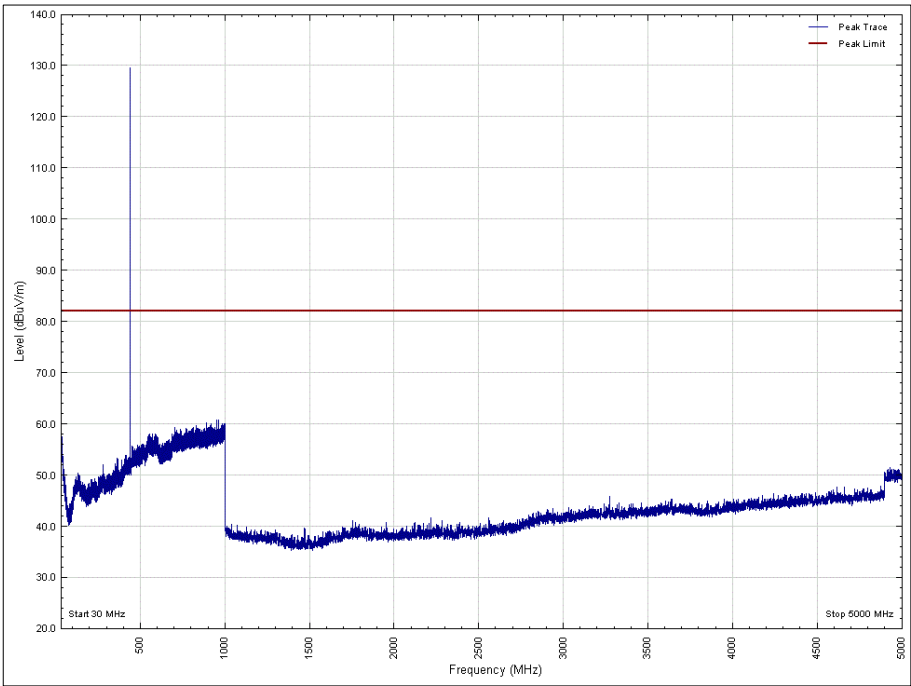
Figure 13 - 438.0500 MHz - 30 MHz to 5 GHz Horizontal, EUT Orientation Z
