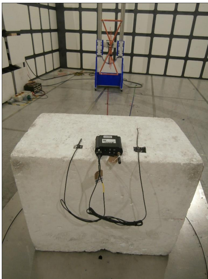
Figure 23 - Test Setup - 30 MHz to 1 GHz, X Orientation
