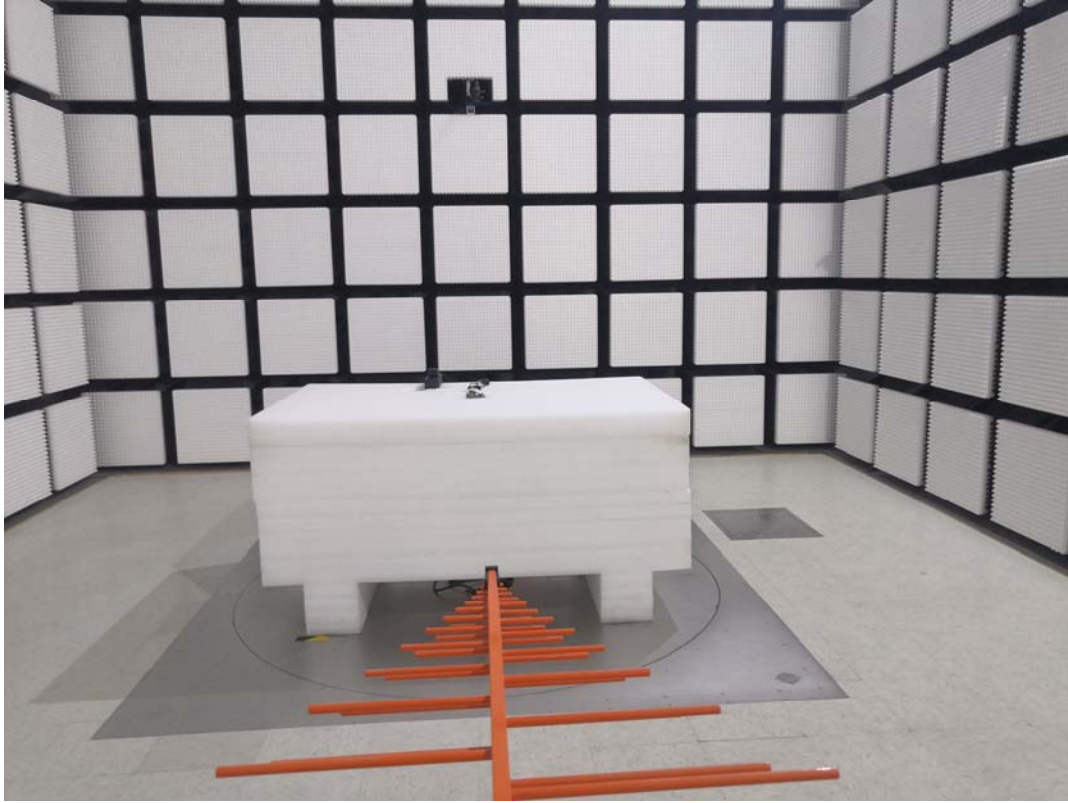
Radiated Emissions Below 1G View-PCB Antenna
