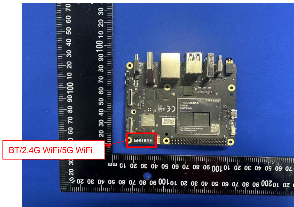
MAIN BOARD TOP VIEW (WITH SHIELDING)
