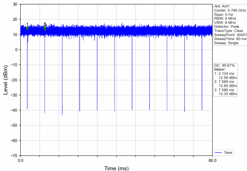
802.11ax(HEW20)_MCH_5785MHz_RU242_Left_Ant1_NTNV
