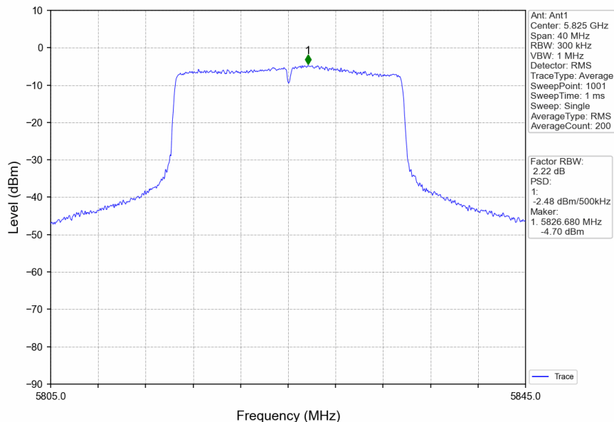
802.11ax(HEW20)_HCH_5825MHz_RU242_Left_Ant1_NTNV
