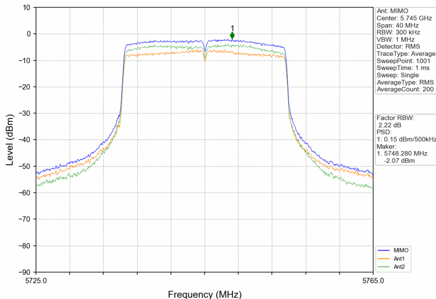
802.11ax(HEW20)_LCH_5745MHz_RU242_Left_MIMO_NTNV
