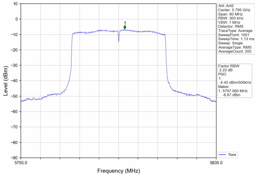
802.11ax(HEW40)_HCH_5795MHz_RU484_Left_MIMO_NTNV
