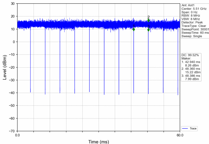
802.11ac(VHT40)_LCH_5510MHz_Ant1_NTNV
