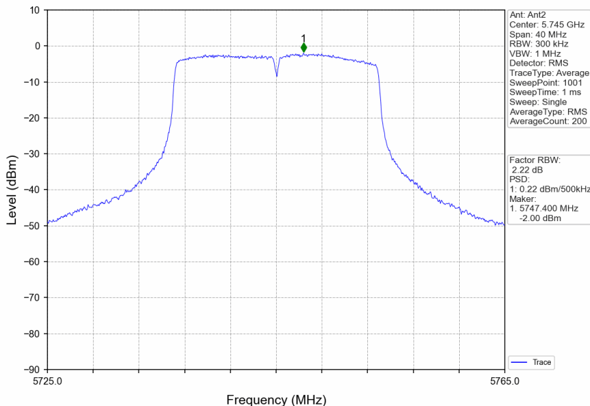
802.11n(HT20)_LCH_5745MHz_Ant2_NTNV
