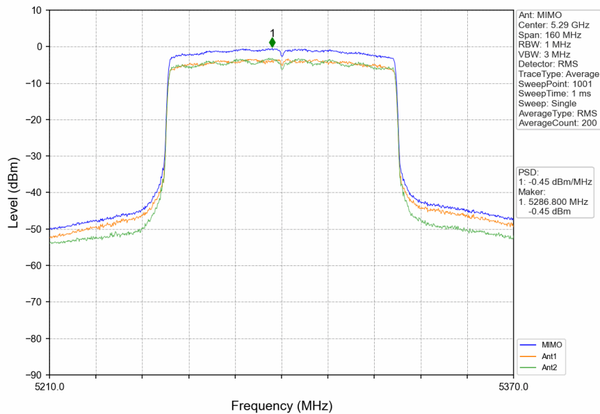
802.11ax(HEW80)_MCH_5290MHz_RU996_Left_MIMO_NTNV
