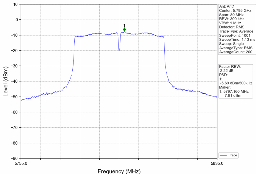
802.11ac(VHT40)_HCH_5795MHz_Ant1_NTNV
