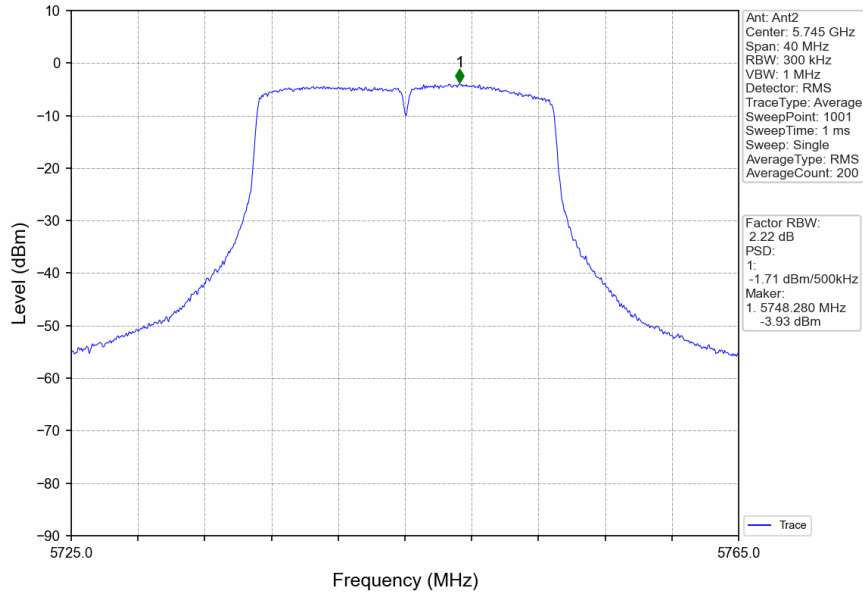
802.11ac(VHT20)_LCH_5745MHz_MIMO_NTNV
