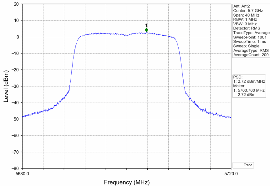
802.11ax(HEW20)_HCH_5700MHz_RU242_Left_Ant2_NTNV
