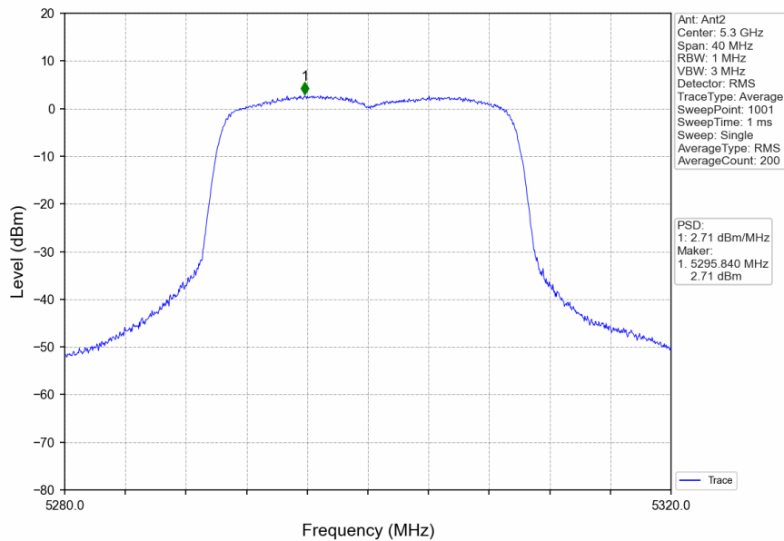
802.11ax(HEW20)_MCH_5300MHz_RU242_Left_Ant2_NTNV
