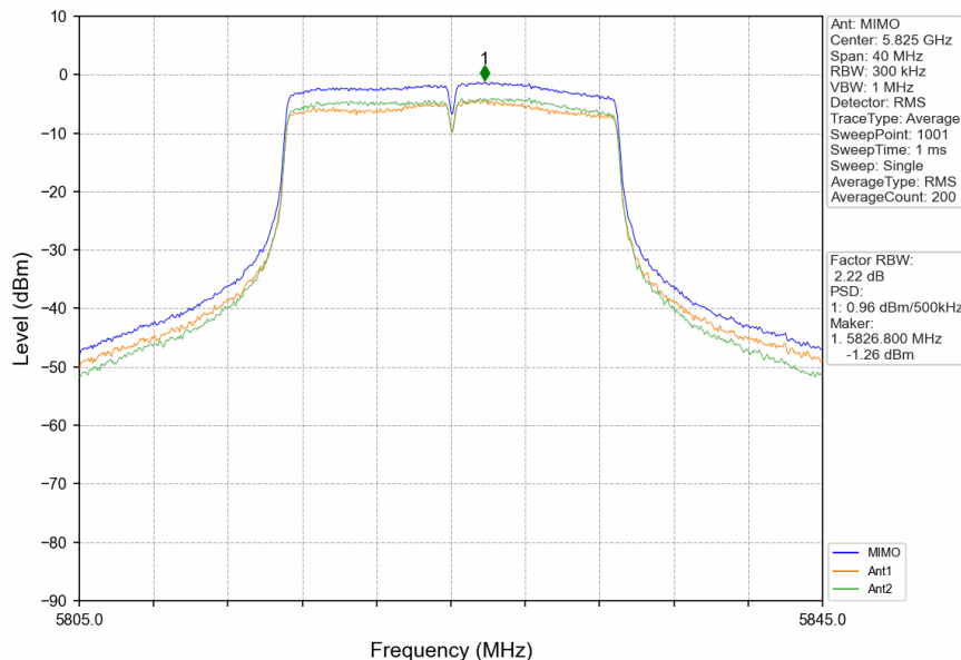
802.11ac(VHT20)_HCH_5825MHz_MIMO_NTNV
