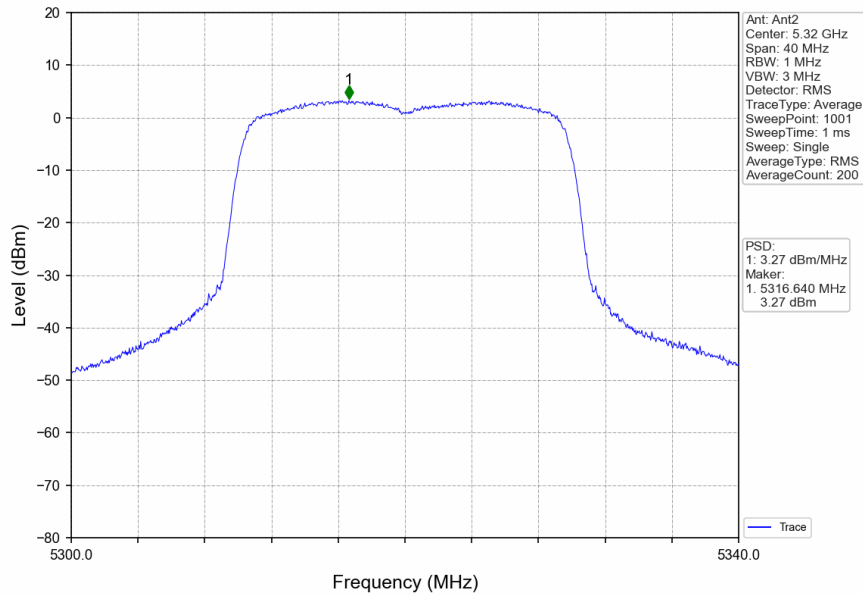
802.11ax(HEW20)_HCH_5320MHz_RU242_Left_MIMO_NTNV
