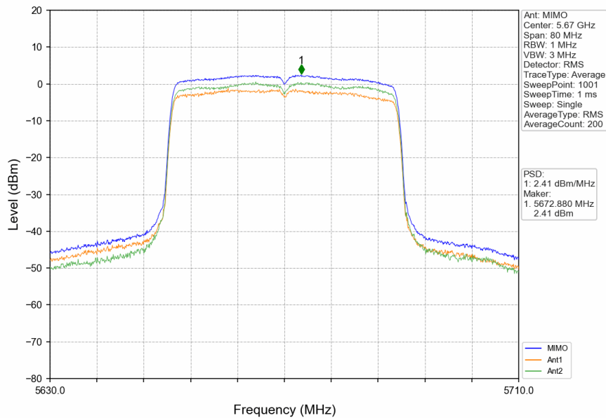
802.11ax(HEW40)_HCH_5670MHz_RU484_Left_MIMO_NTNV
