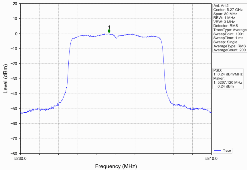
802.11ax(HEW40)_LCH_5270MHz_RU484_Left_MIMO_NTNV
