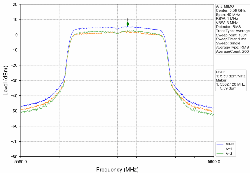
802.11ax(HEW20)_MCH_5580MHz_RU242_Left_MIMO_NTNV
