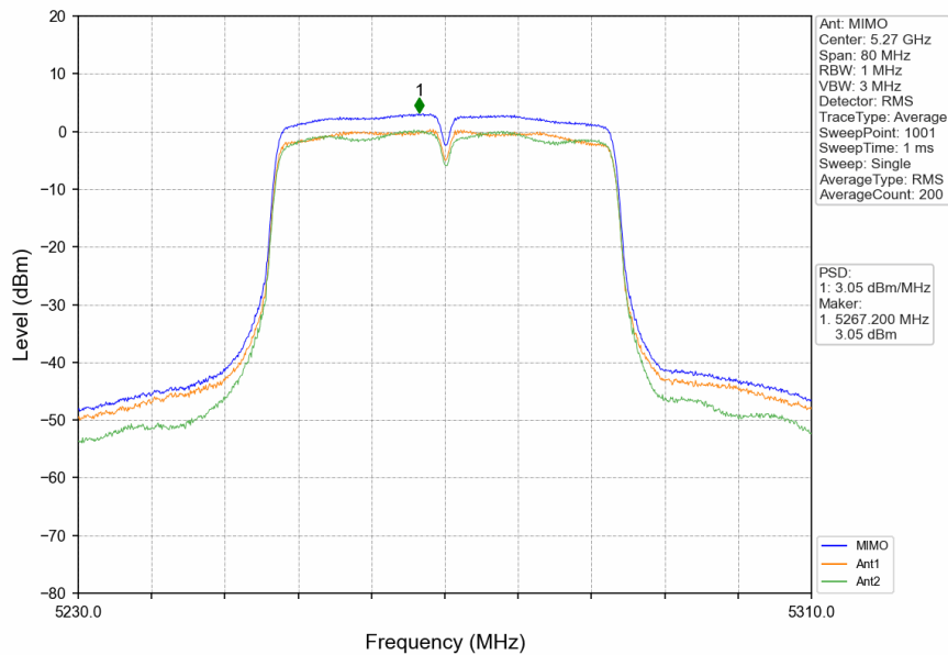
802.11ac(VHT40)_LCH_5270MHz_MIMO_NTNV
