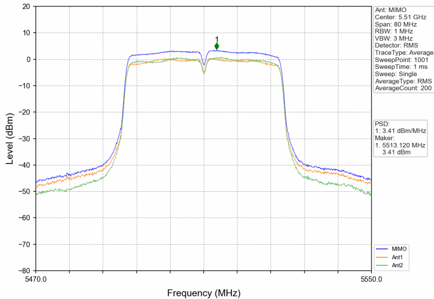
802.11ac(VHT40)_LCH_5510MHz_MIMO_NTNV
