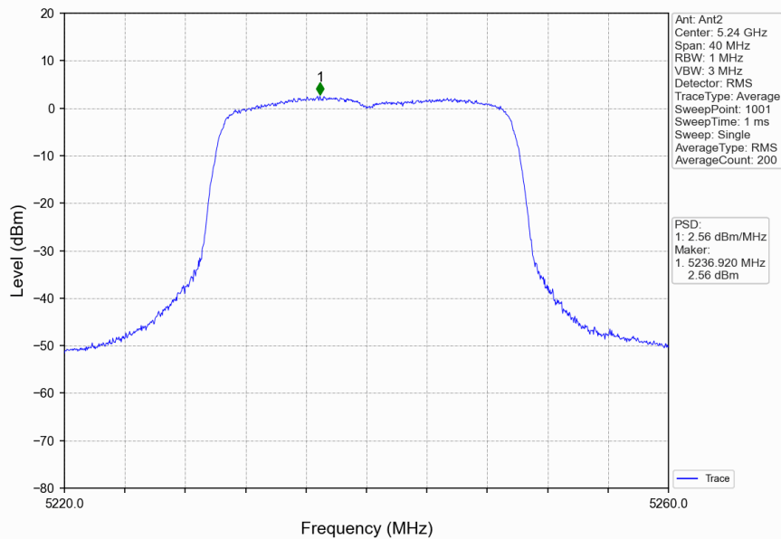
802.11ax(HEW20)_HCH_5240MHz_RU242_Left_Ant2_NTNV
