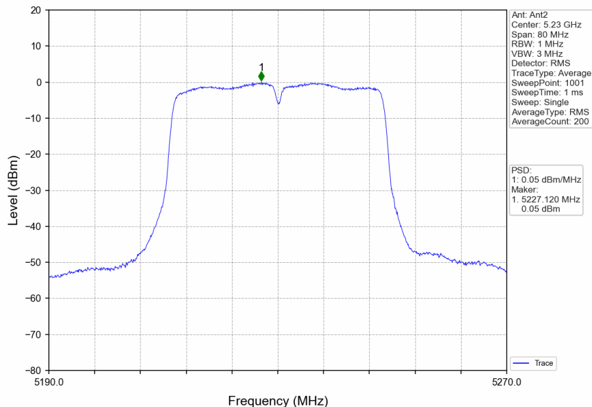
802.11ac(VHT40)_HCH_5230MHz_Ant2_NTNV
