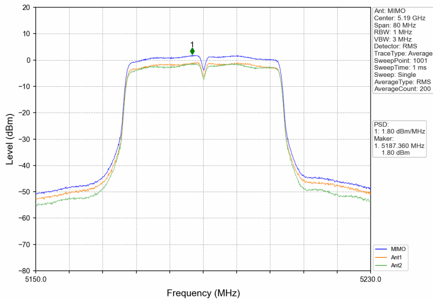
802.11ac(VHT40)_LCH_5190MHz_MIMO_NTNV
