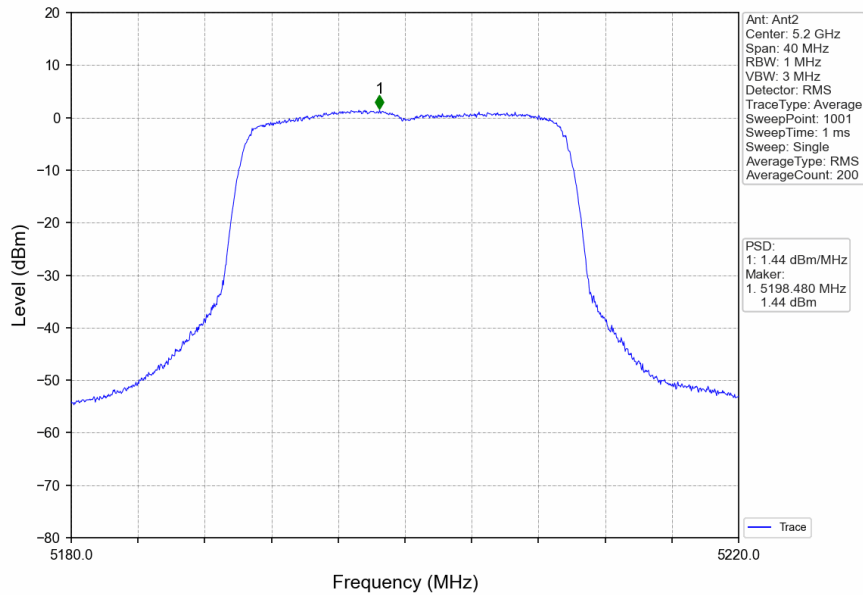
802.11ax(HEW20)_MCH_5200MHz_RU242_Left_MIMO_NTNV
