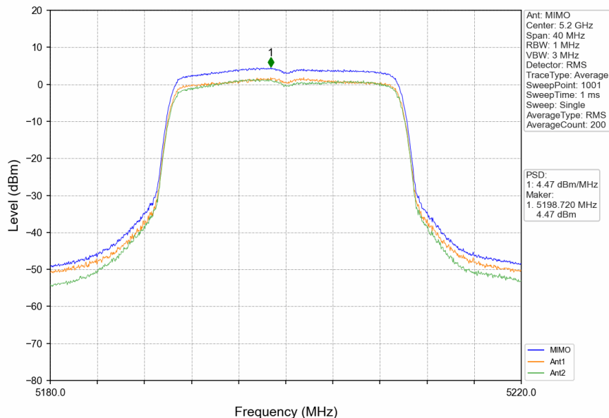
802.11ax(HEW20)_MCH_5200MHz_RU242_Left_MIMO_NTNV
