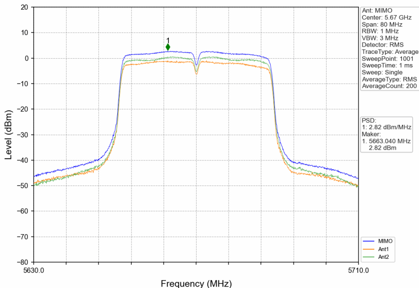
802.11ac(VHT40)_HCH_5670MHz_MIMO_NTNV
