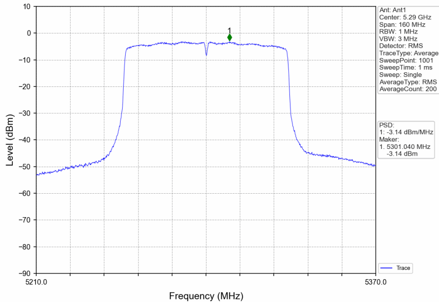
802.11ac(VHT80)_MCH_5290MHz_Ant1_NTNV
