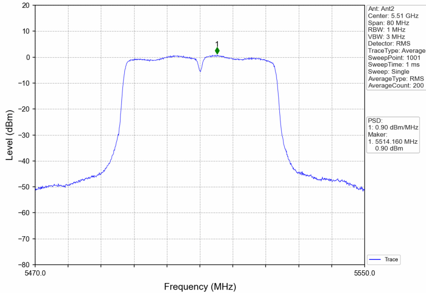
802.11ac(VHT40)_LCH_5510MHz_MIMO_NTNV
