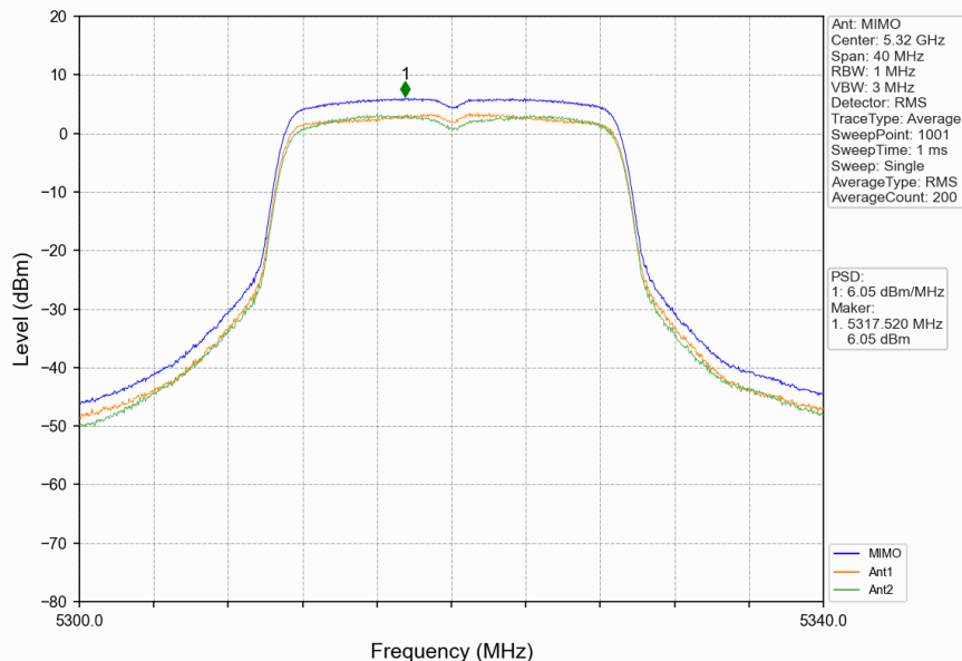
802.11ac(VHT20)_HCH_5320MHz_MIMO_NTNV
