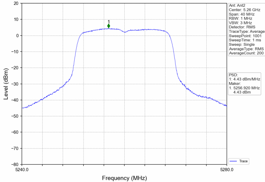
802.11n(HT20)_LCH_5260MHz_MIMO_NTNV
