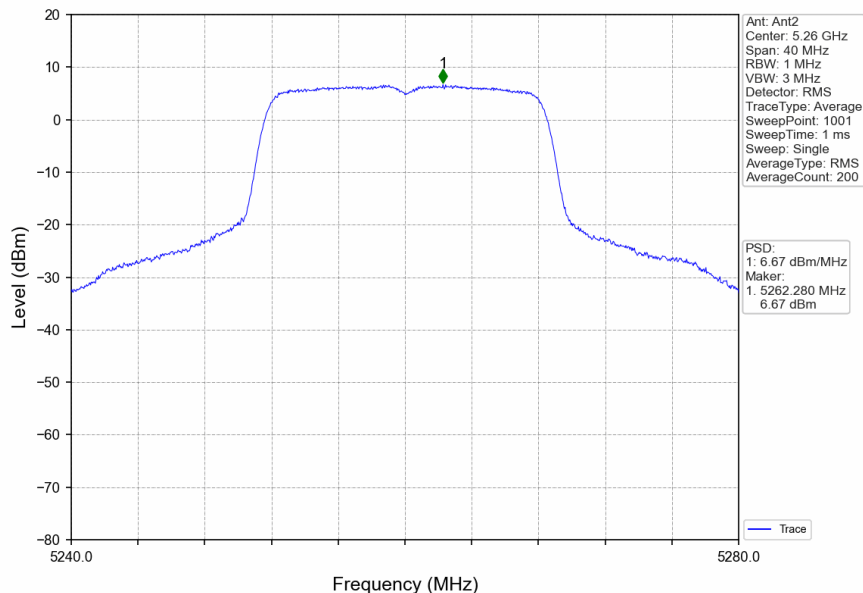
802.11a_LCH_5260MHz_Ant2_NTNV
