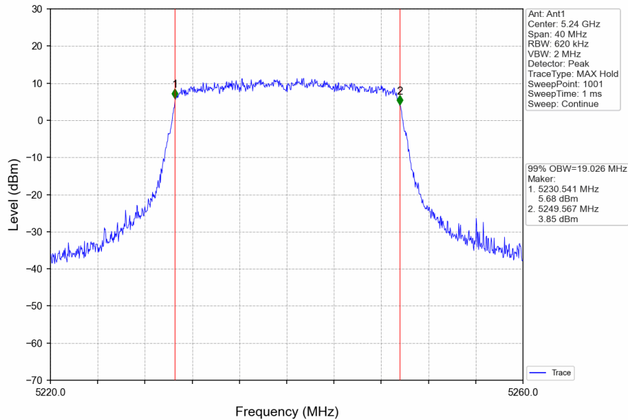
802.11ax(HEW20)_HCH_5240MHz_RU242_Left_Ant1_NTNV
