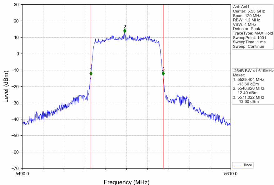
802.11ax(HEW40)_MCH_5550MHz_RU484_Left_Ant1_NTNV
