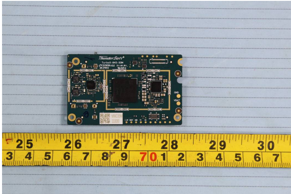
EUT –RF Board 3 Top View
