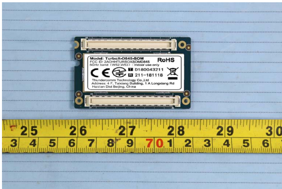
EUT –RF Board 1 Bottom View
