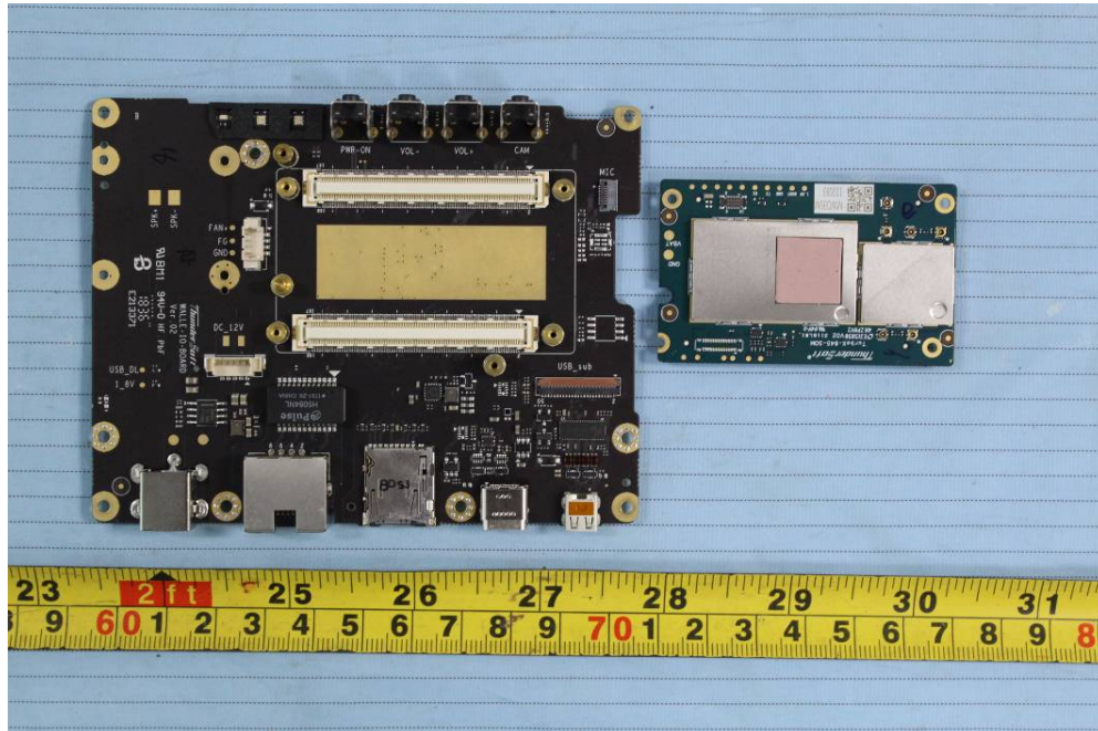
EUT – Main Board Top Shilding off View 2
