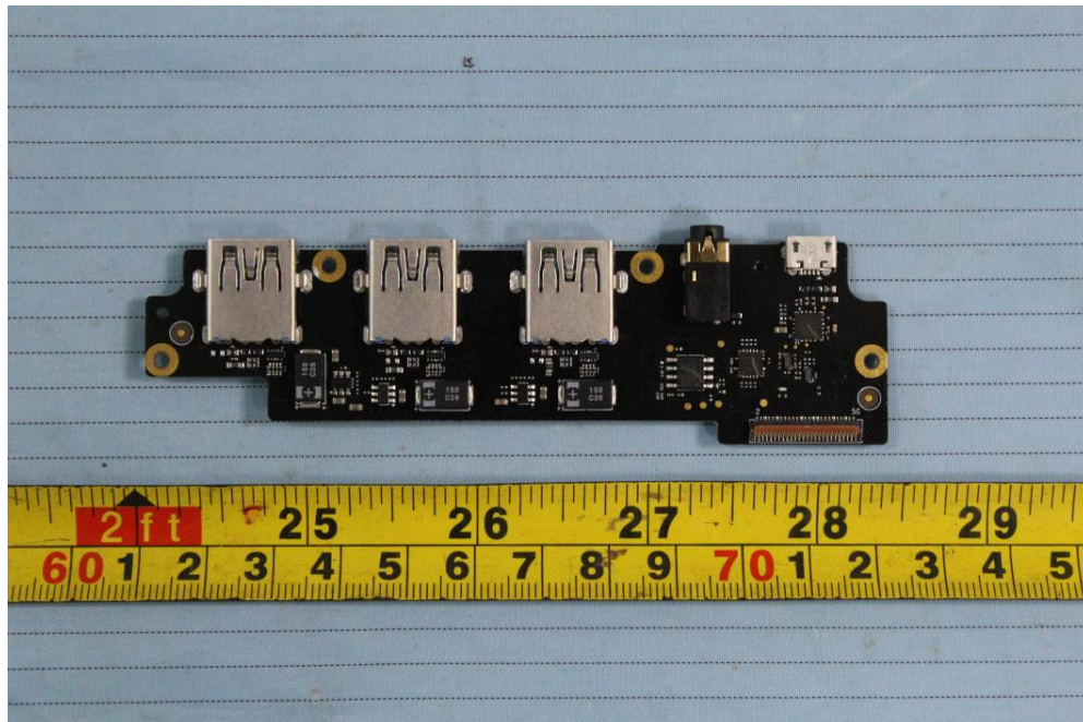
EUT –USB Board Top View
