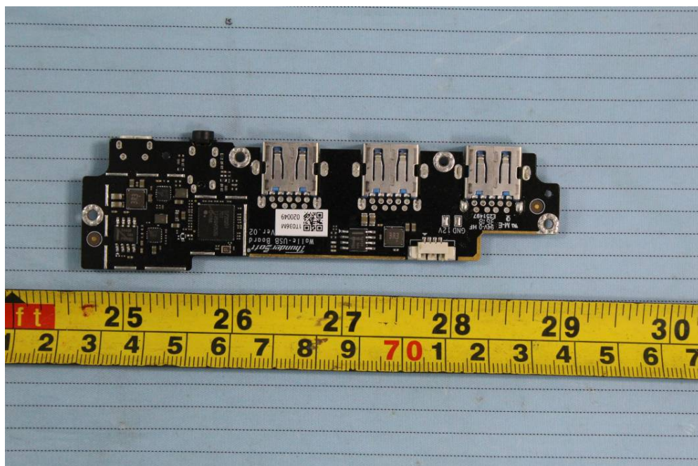
EUT –USB Board Bottom View
