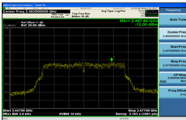
802.11g CH-High
