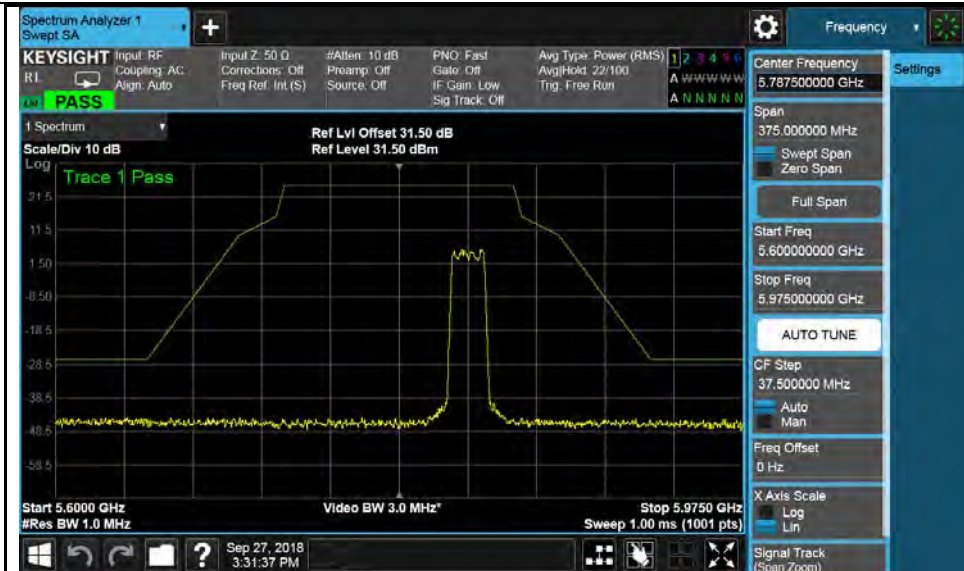
802.11ac-VHT20-5825MHz
