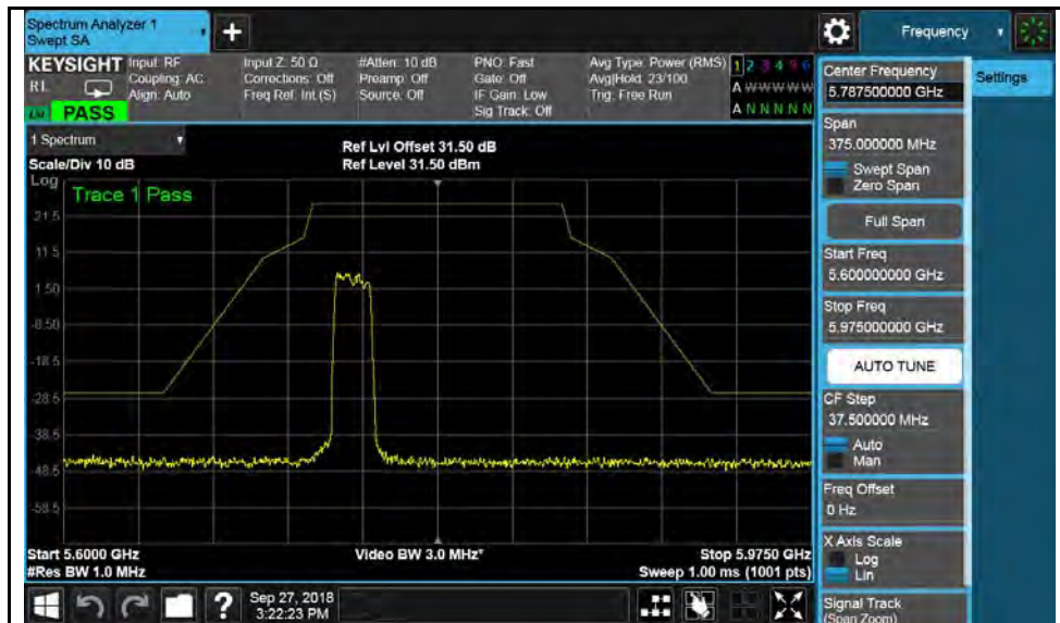
802.11ac-VHT20-5745MHz
