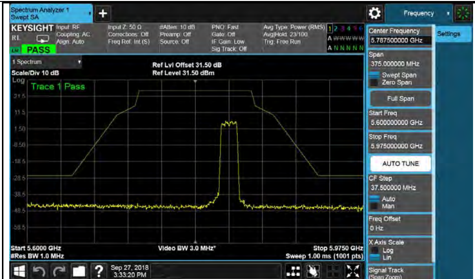
802.11ac-VHT20-5825MHz
