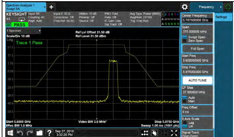
802.11ac-VHT20-5825MHz
