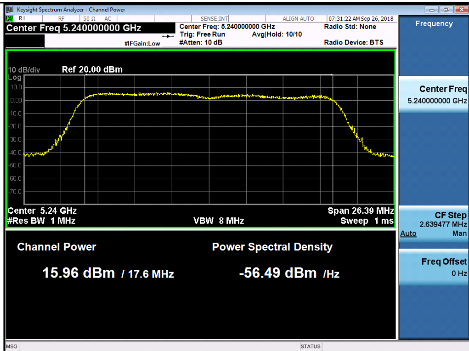
802.11ac20 5240M
