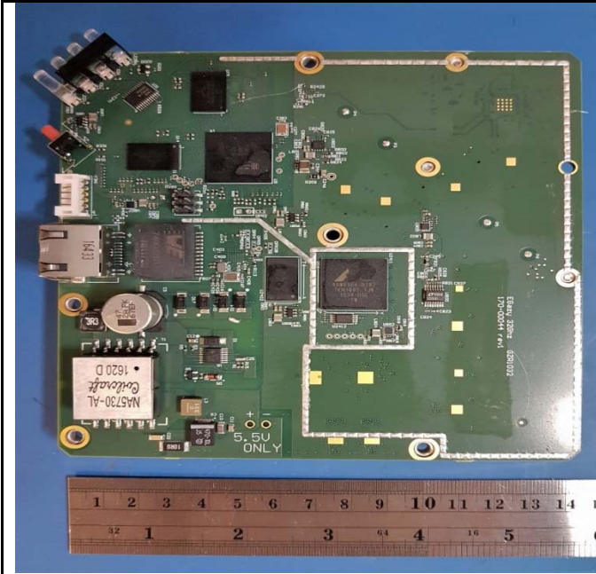
Internal-Gazer-32G-BackSide- PCB
