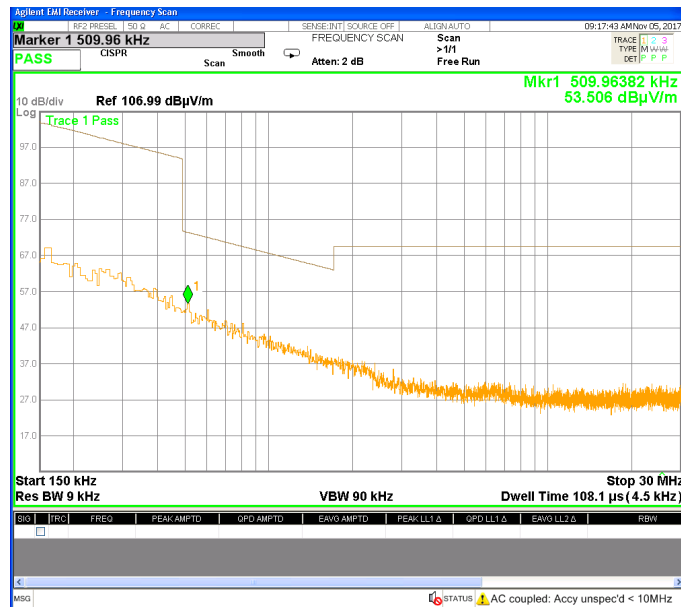
Plot # 26. Investigation result in 0.15 – 30 MHz frequency range.
