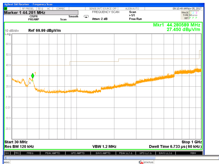
Plot # 27. Investigation result in 30 - 1000 MHz frequency range.
