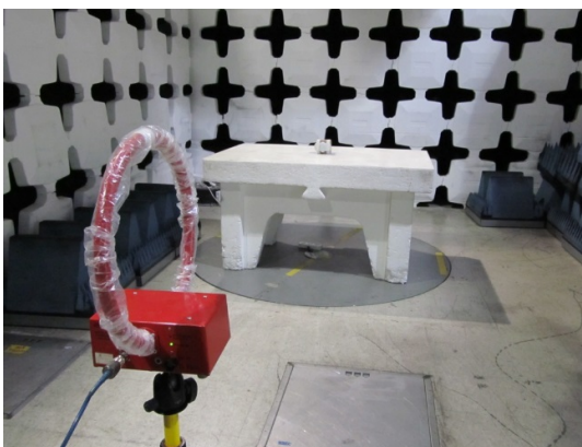
Radiated emissions test set up below 30MHz.
