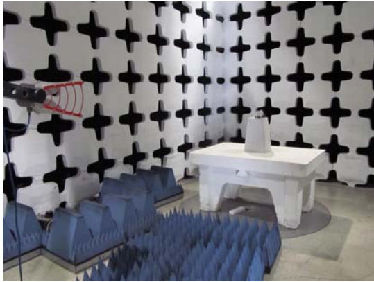
Radiated emissions test set up above 1GHz.
