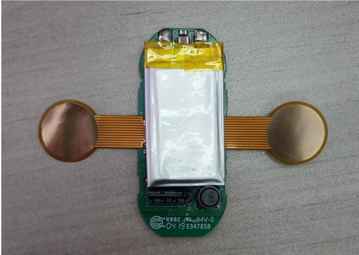
BOTTOM SIDE WITH SWITCH, FLEX PCB AND BATTERY
