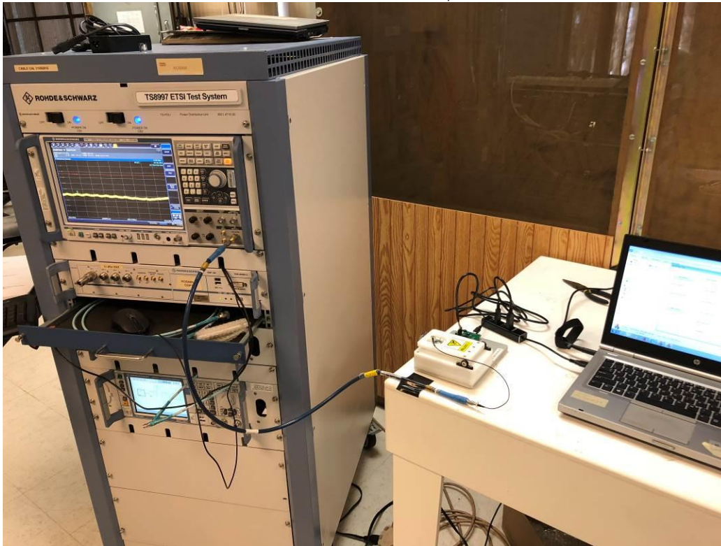
Antenna Port Conducted Emissions, 30-25000 MHz
