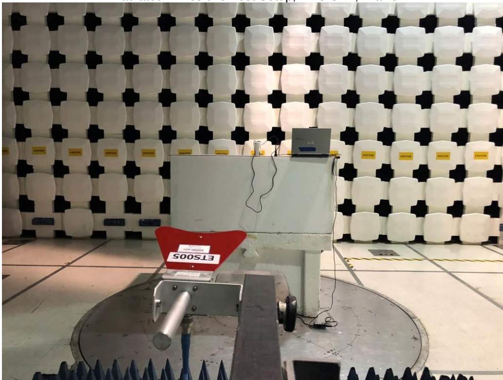
Radiated Emissions Test Setup, 1-18 GHz, Y-axis
