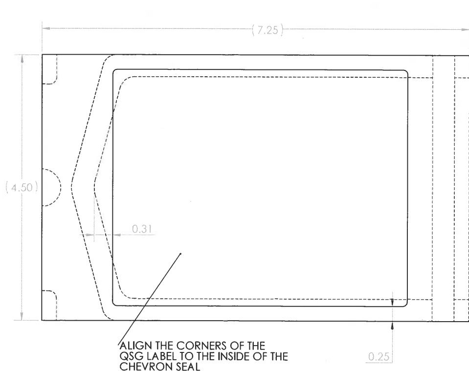
BOTTOM VIEW
