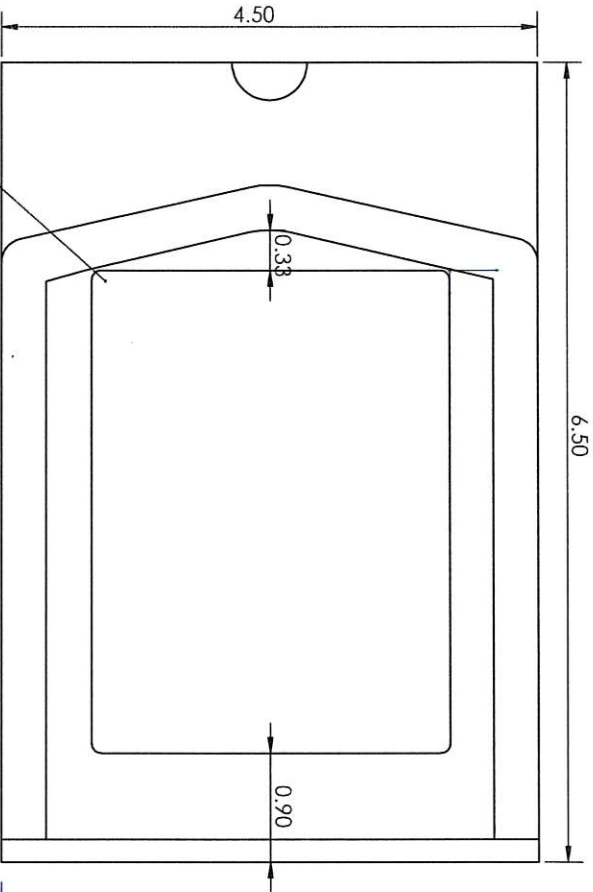
TOP VIEW: CLEAR PET SIDE
