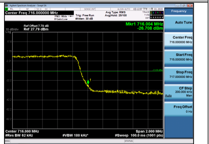
HCH_16QAM_15RB#0
