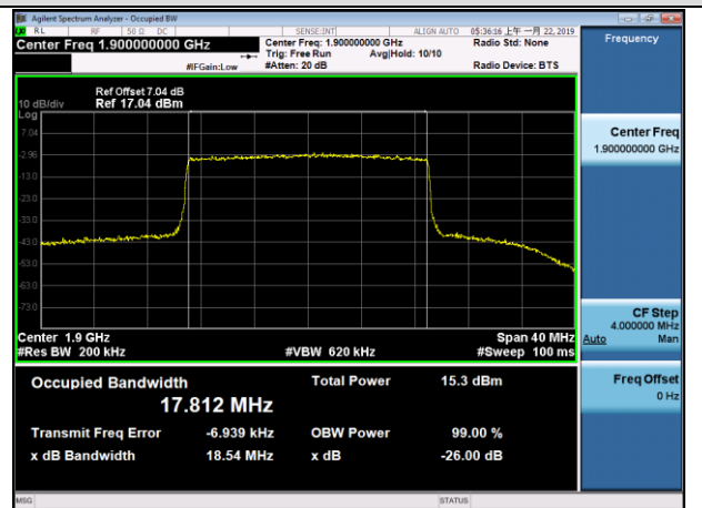
HCH_16QAM_100RB#0
