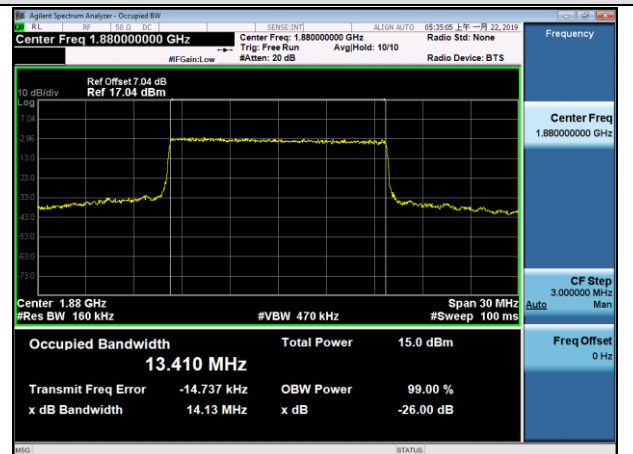
MCH_16QAM_75RB#0
