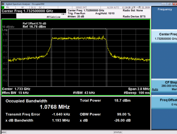
MCH_QPSK_6RB#0
