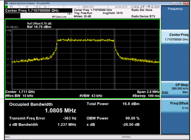
LCH_16QAM_6RB#0
