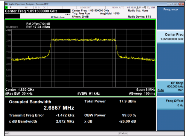
LCH_16QAM_15RB#0
