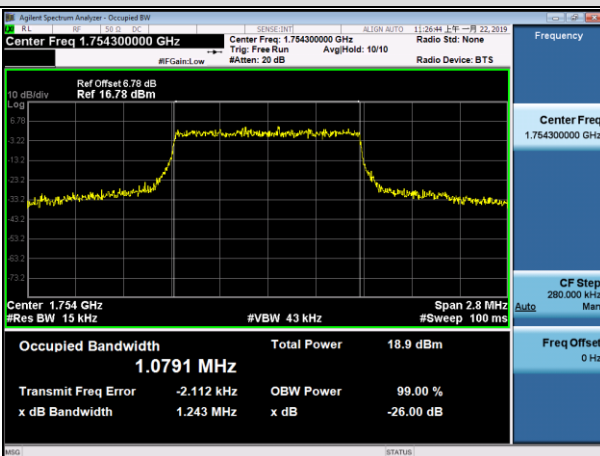
HCH_QPSK_6RB#0
