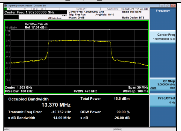
HCH_16QAM_75RB#0
