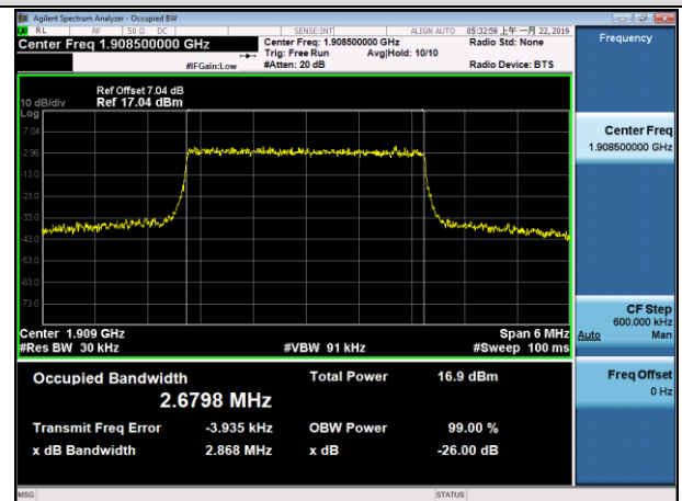
HCH_16QAM_15RB#0
