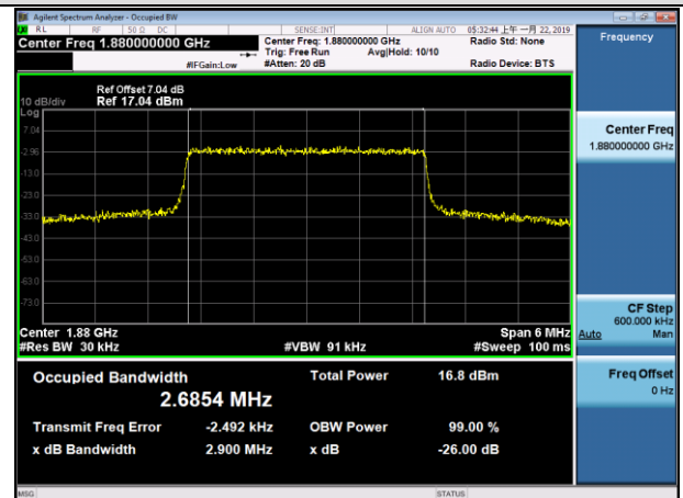
MCH_16QAM_15RB#0
