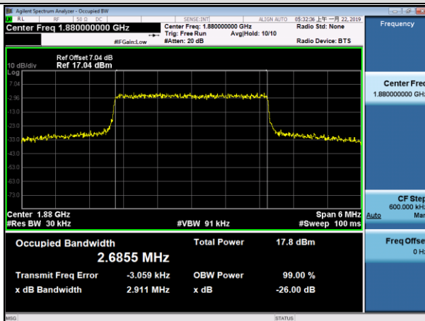
MCH_QPSK_15RB#0
