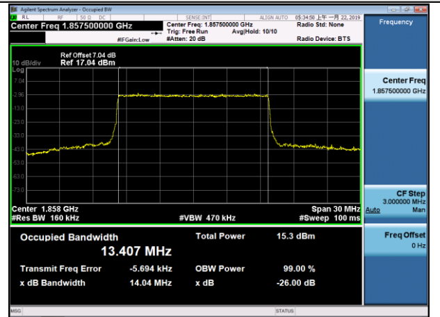
LCH_16QAM_75RB#0
