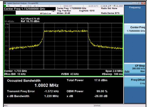
MCH_16QAM_6RB#0
