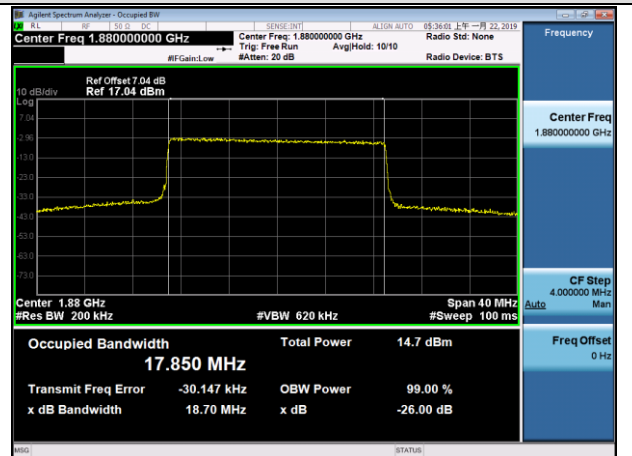
MCH_16QAM_100RB#0
