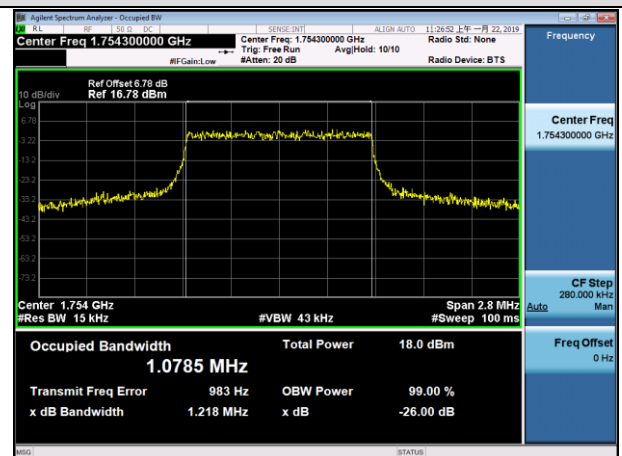
HCH_16QAM_6RB#0
