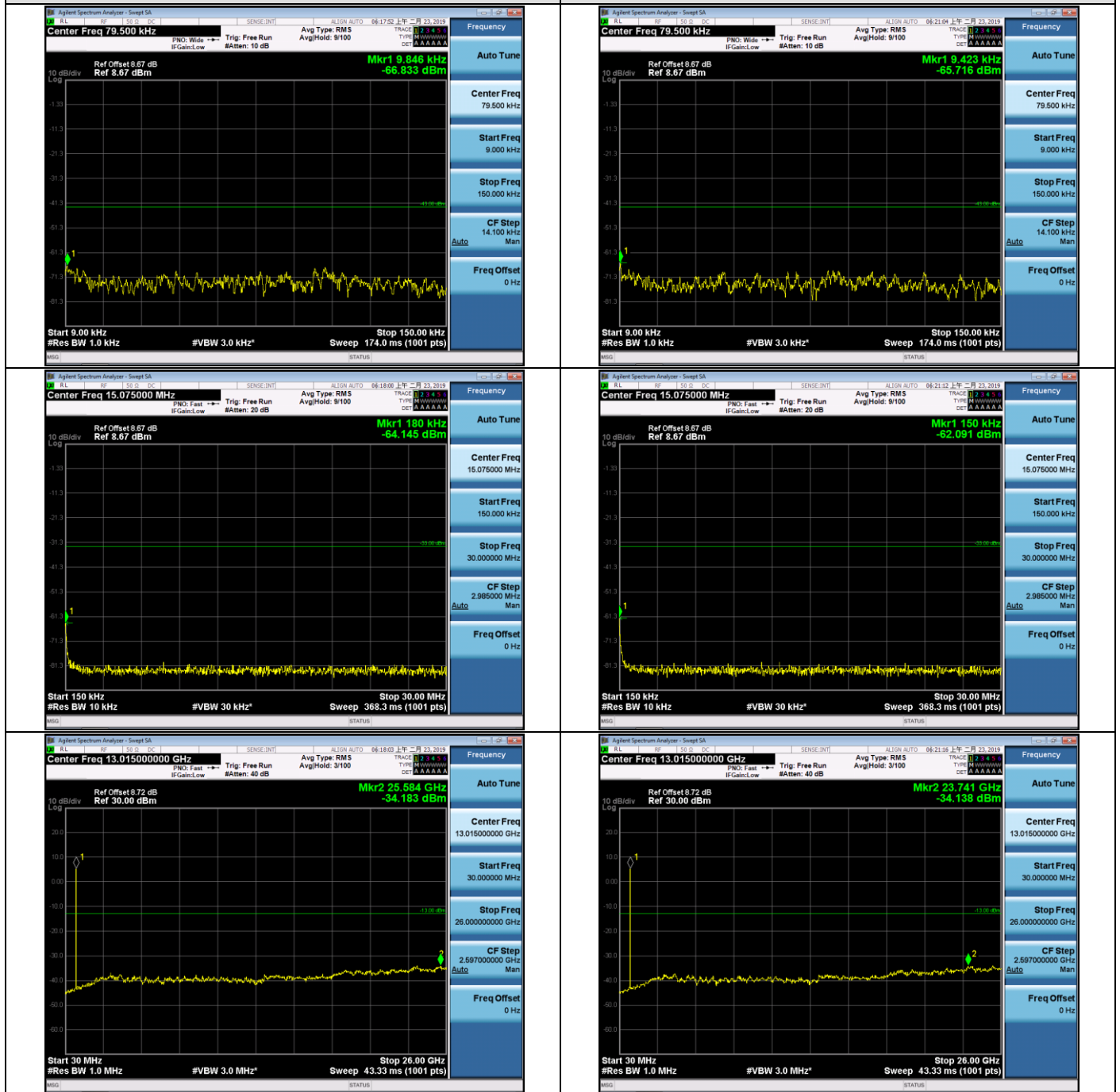
5MHz_LCH_QPSK_1RB#0
