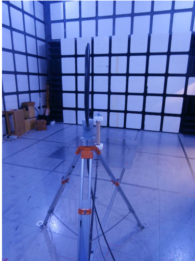
Radiated Emissions Edge On
