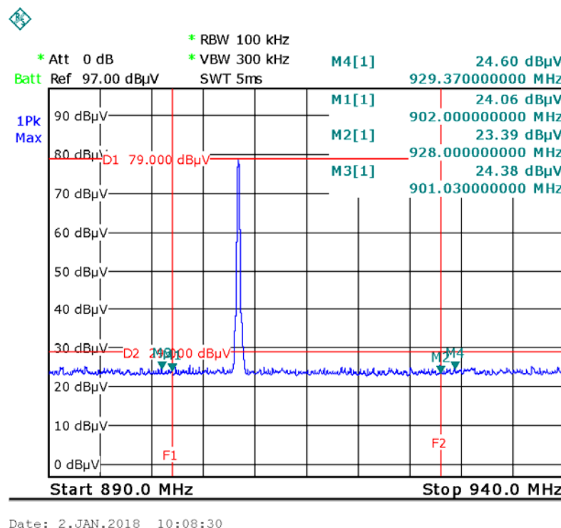
Test plots
