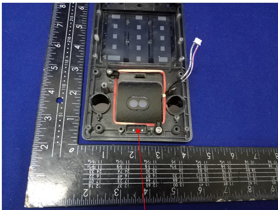
125KHz Antenna
