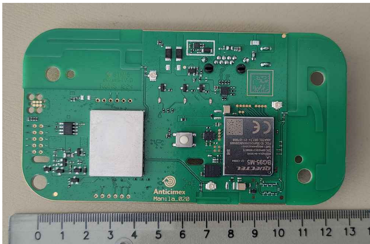
EUT PCB from front side
