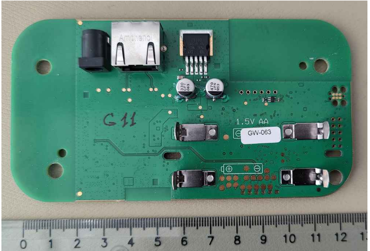
EUT PCB from bottom side
