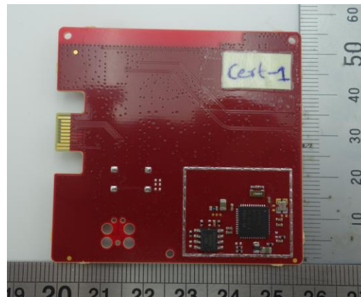
Copa-Cell board – Back side
