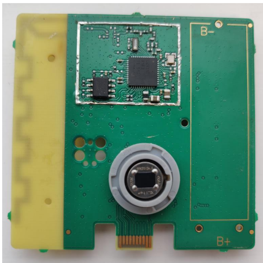
Without shieldcan
