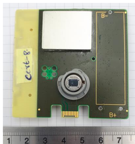
Copa-Mesh board – Back side
