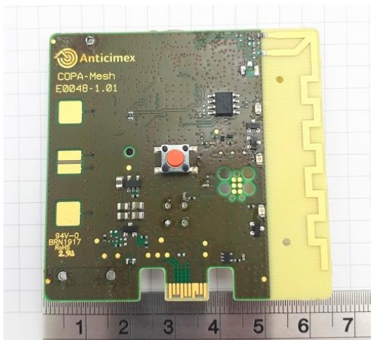
Copa-Mesh board – Front side
