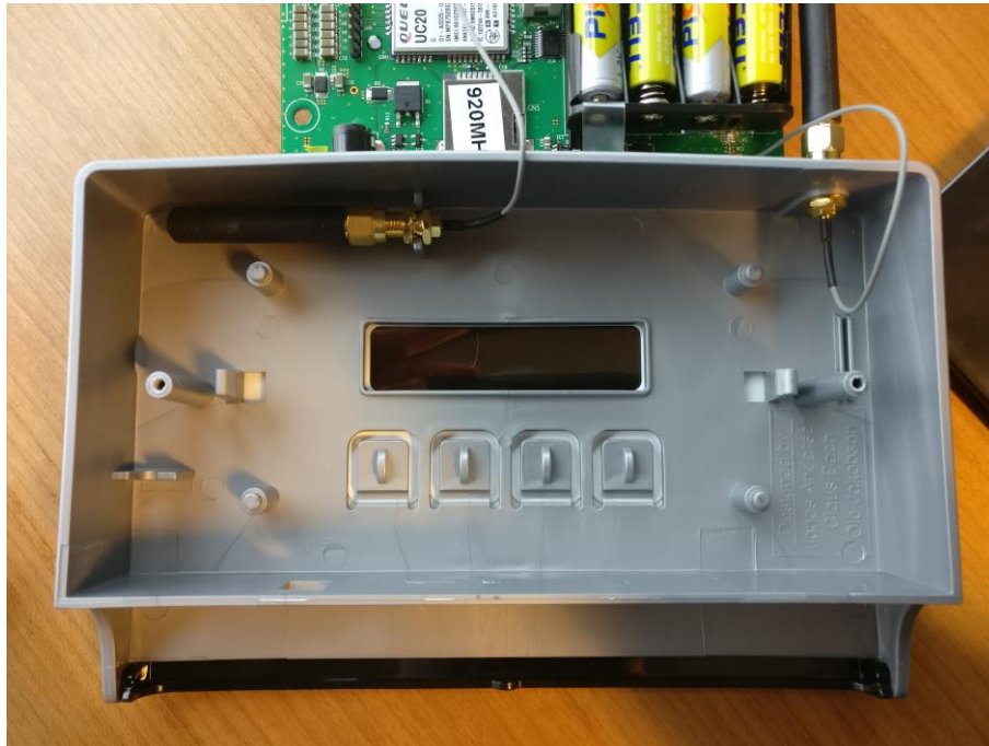
Figure 5: Inside of main enclosure without PCB attached.
