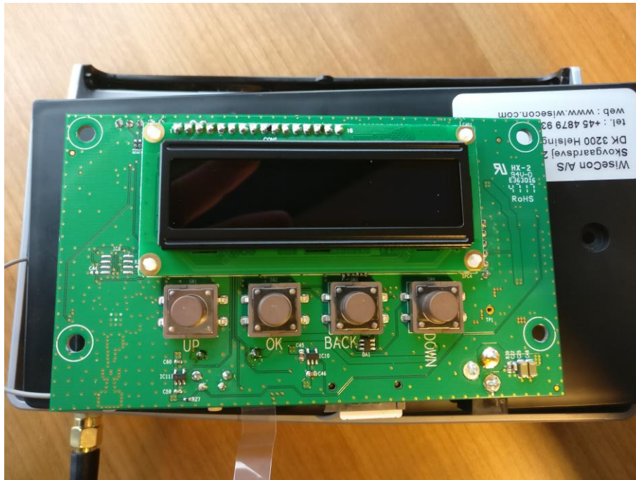
Figure 3: Shows the front side of the PCB
