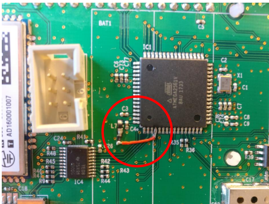
Figure 4: Shows modifications done to the back side of the PCB (under battery holder). 3.3V supply wire added to 510k ohm pull up. See document "13 Smart Eye Schem.pdf" for schematic of modification.
