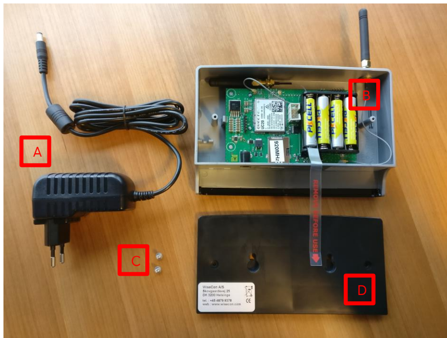
Figure 1: Shows the main parts of the Smart Connect. A) power supply, B) main enclosure, C) screws for enclosure back and D) enclosure back panel
