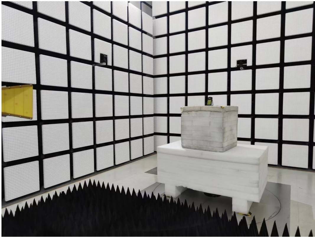
Radiated Emission 18G-26.5GHz View
