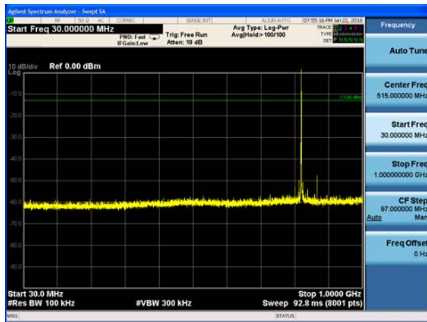
NB-IOT Band 5 CH-Middle 30MHz-1GHz
