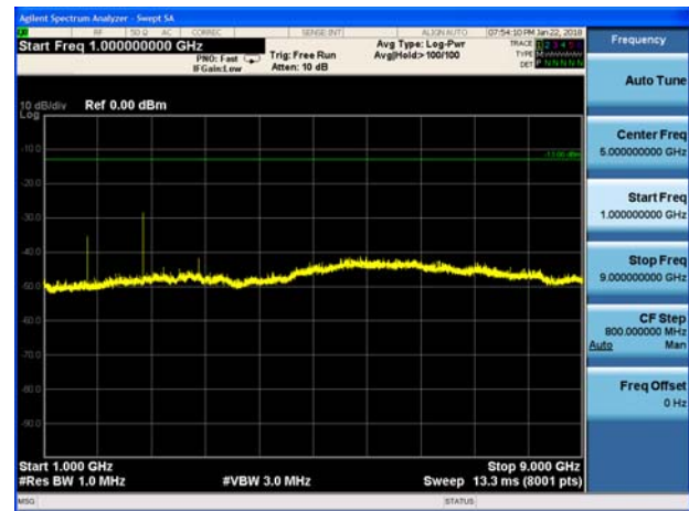
NB-IOT Band 5 CH-Middle 1GHz-9GHz
