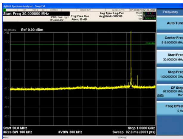
NB-IOT Band 5 CH-High 30MHz-1GHz
