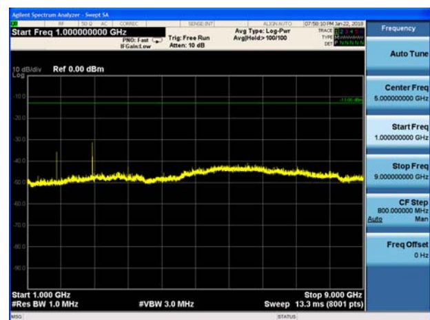
NB-IOT Band 5 CH-High 1 GHz-9GHz
