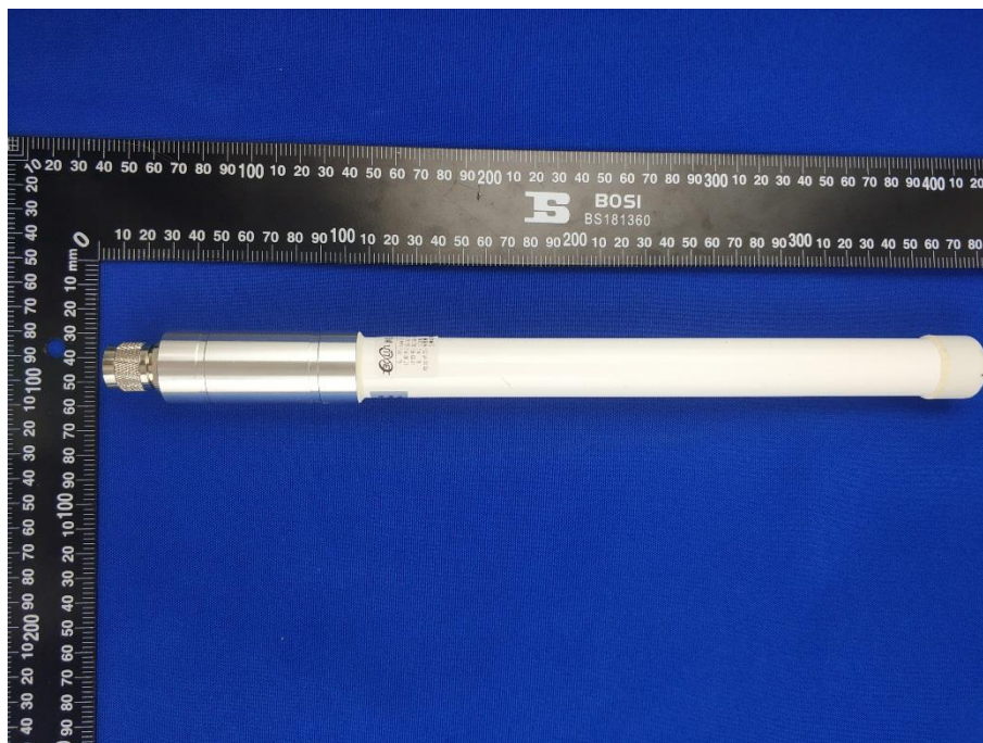
Accessory-Lora Antenna
