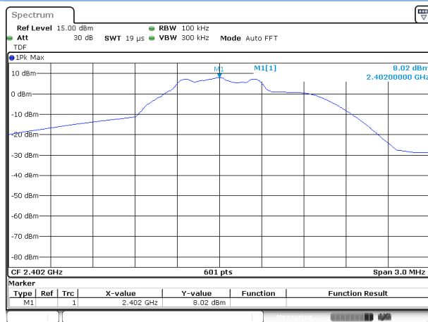
GFSK (BLE) LOW CHANNEL , CARRIER LEVEL
