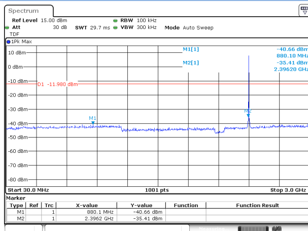
GFSK (BLE) LOW CHANNEL , SPURIOUS 30 MHz ~ 3 GHz
