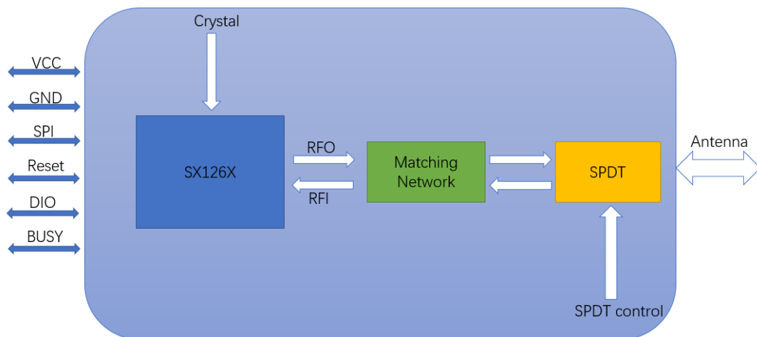
Figure 2 Hardware system block diagram
