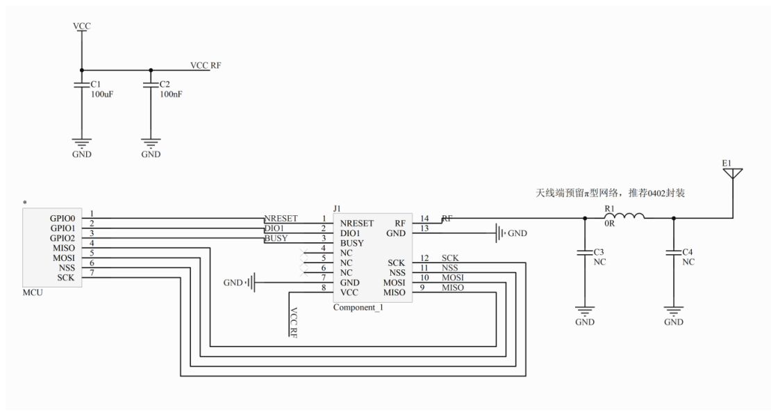
Figure 3 Typical application circuit
