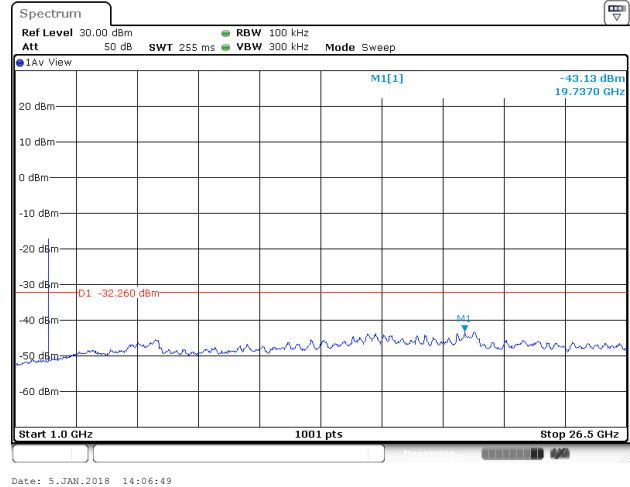
802.11g on channel 01
