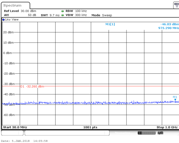
802.11g on channel 01
