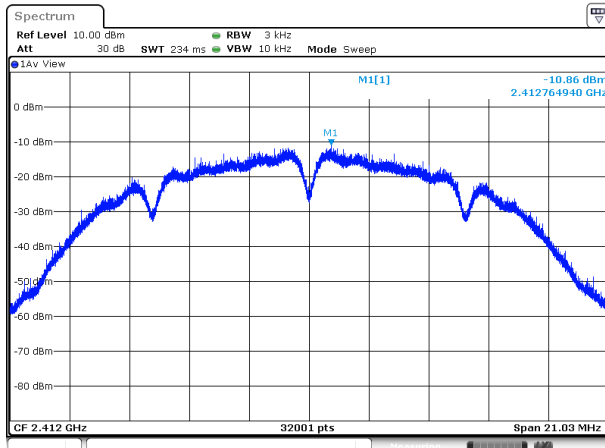
(802.11b) PSD plot on channel 1
