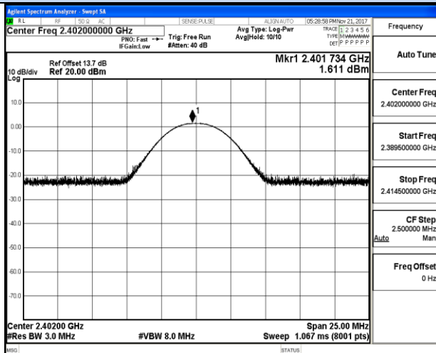
Channel 0 / 2402 MHz
