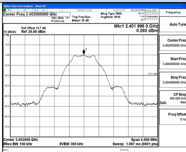
Channel 0 / 2402 MHz
