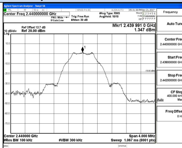
Channel 19 / 2440 MHz
