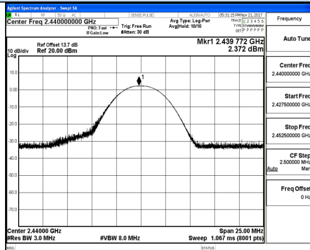
Channel 19 / 2440 MHz
