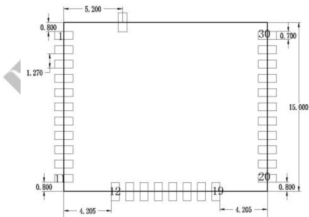
Figure 2-2 Product package diagram
