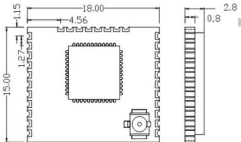
Figure 2-1 Dimensions
