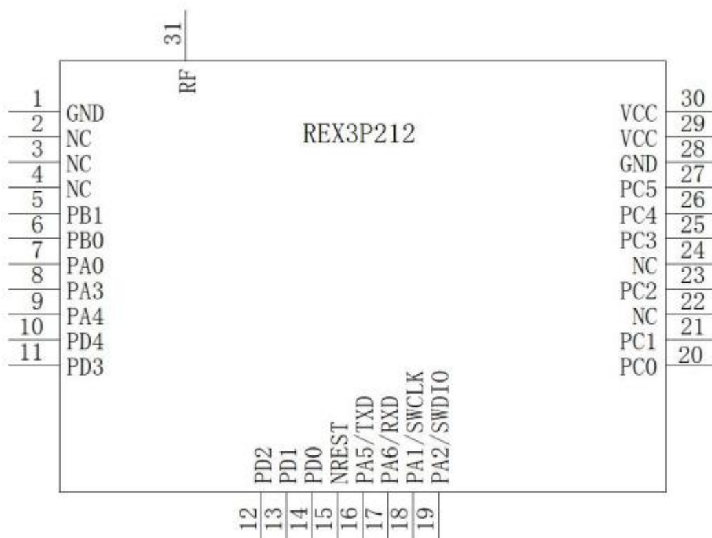
Figure 2-3 Pin configuration diagram
