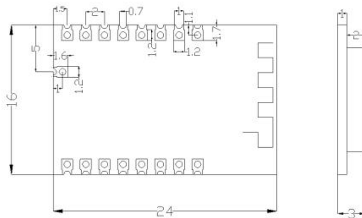
Figure2-1 Dimensions
