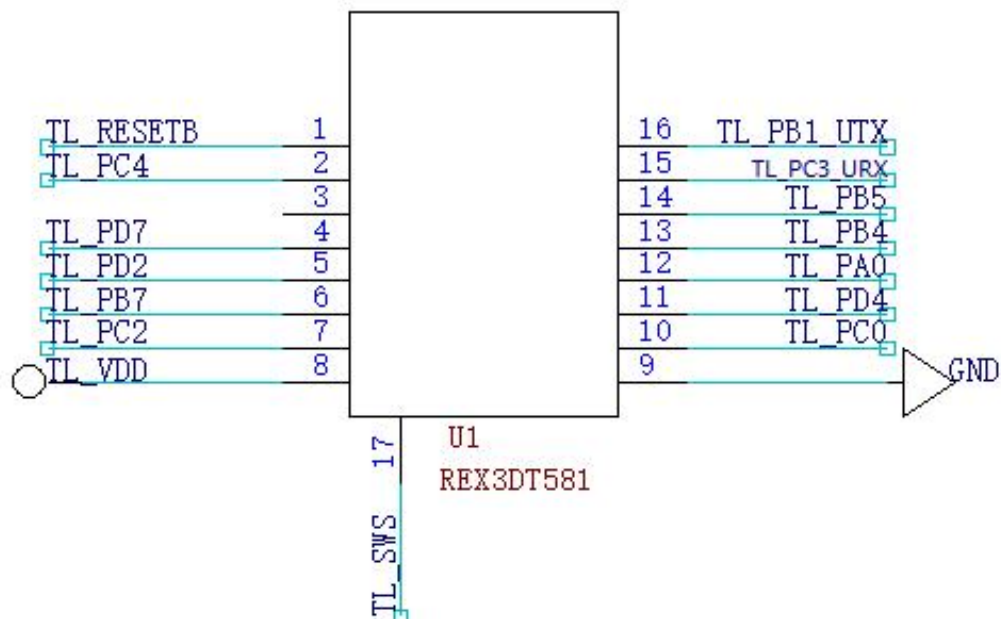
Figure2-3 Pin Configuration
