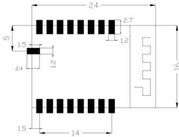
Figure2-2 Packaging
