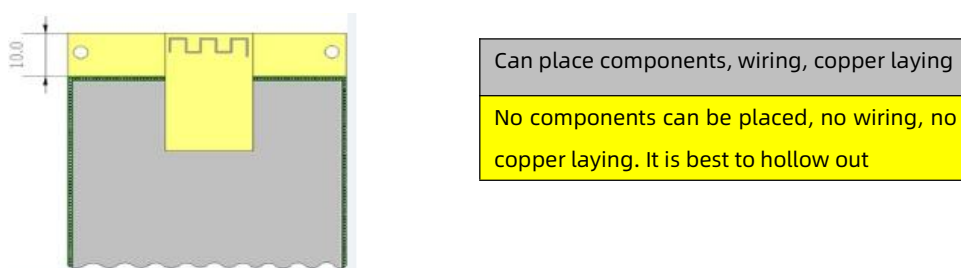
Figure 5-1 PCB layout diagram for module antenna position selection
