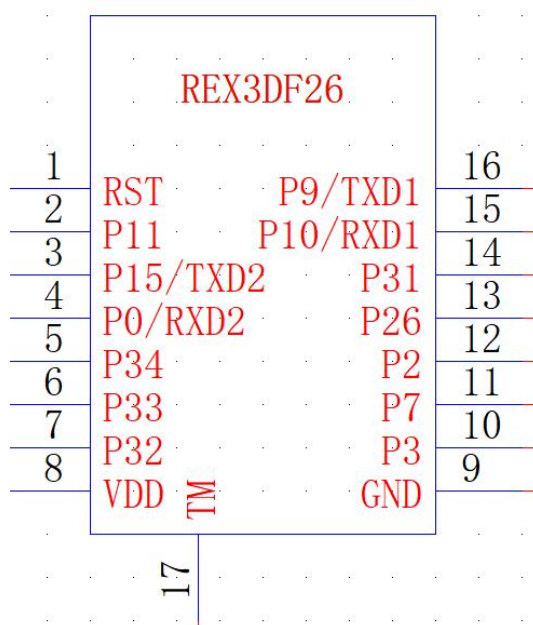
Figure 2-3 Pin configuration diagram
