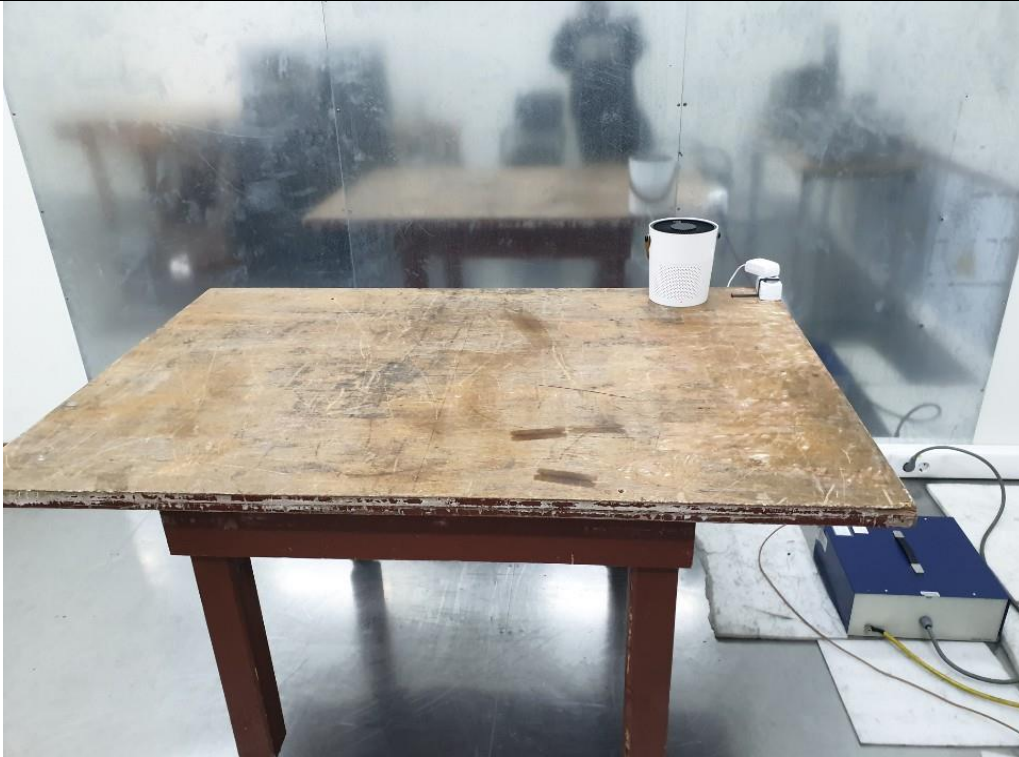
AC Power Line Conducted Emission Test 1
