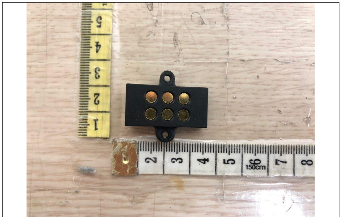
PCB 2 (Bottom)
