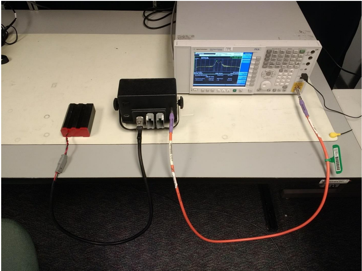
Figure 5: RF Conducted Test Setup
