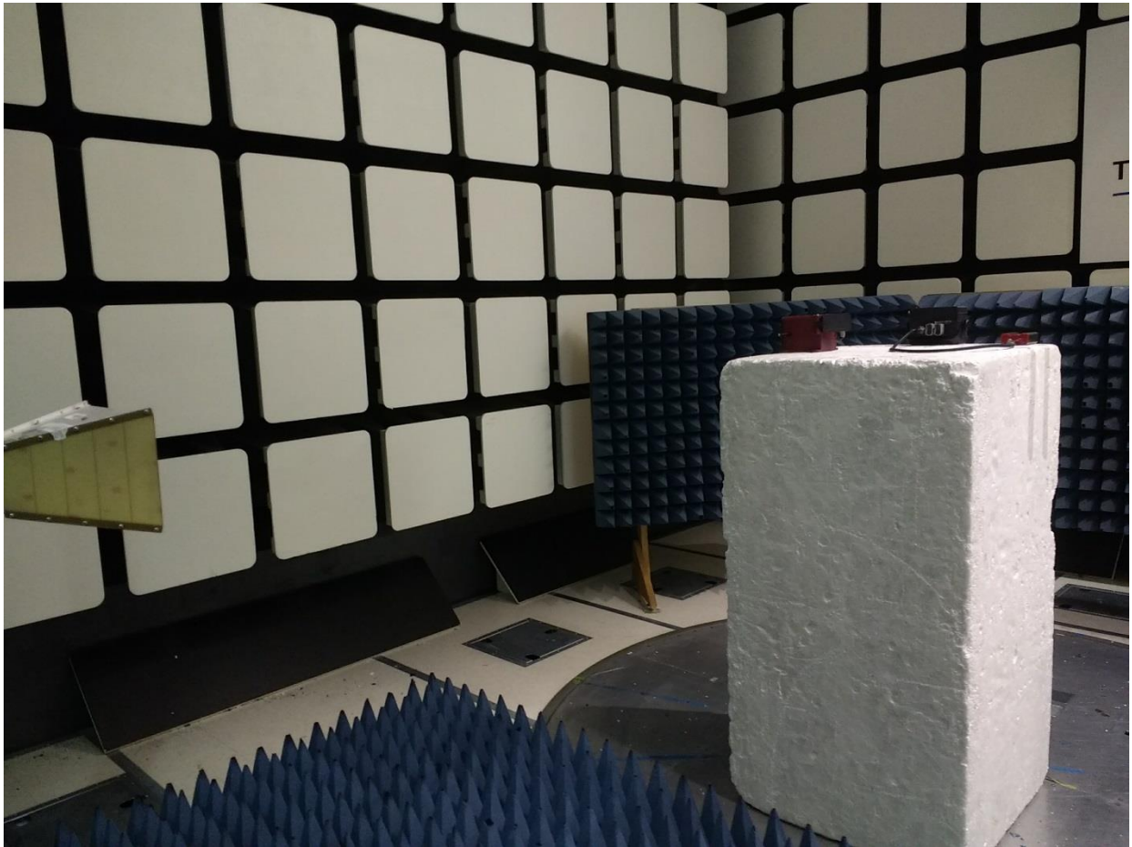
Figure 3: Test Setup for 1GHz to 10GHz (Front View)
