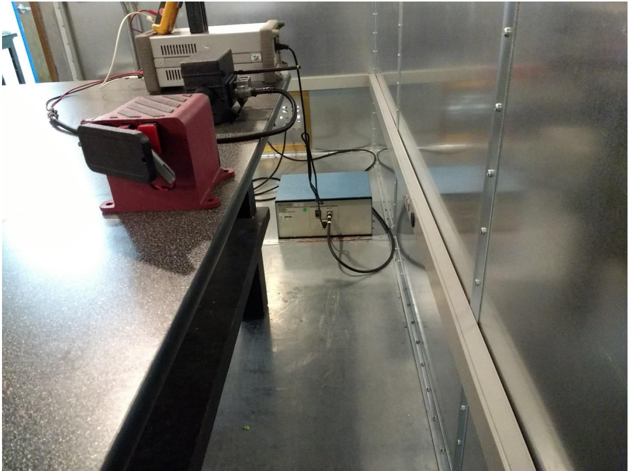
Figure 7: Conducted Emission Test Setup (Side)
