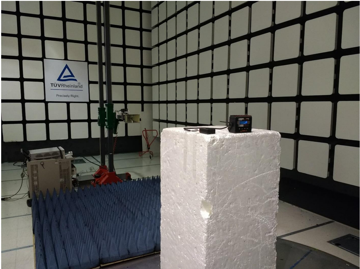
Figure 4: Test Setup for 1GHz to 10GHz (Rear View)
