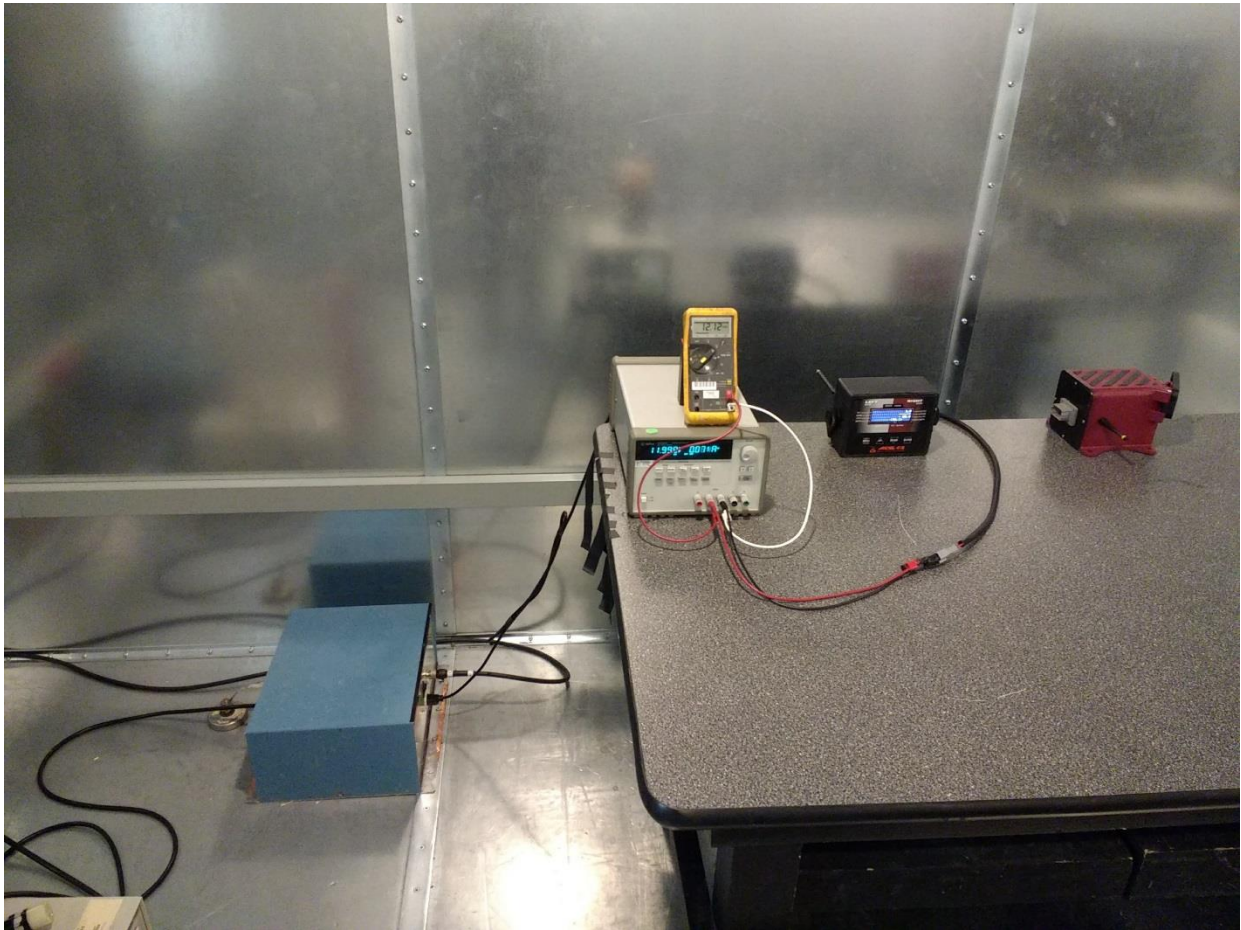
Figure 6: Conducted Emission Test Setup (Front)
