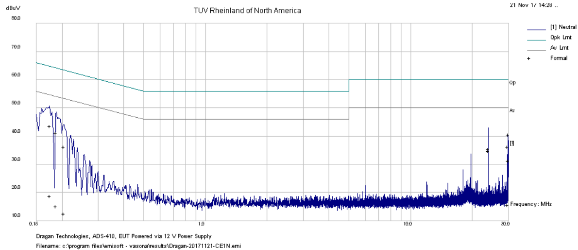
150 kHz to 30 MHz Plot for Line 2 (Neutral)
